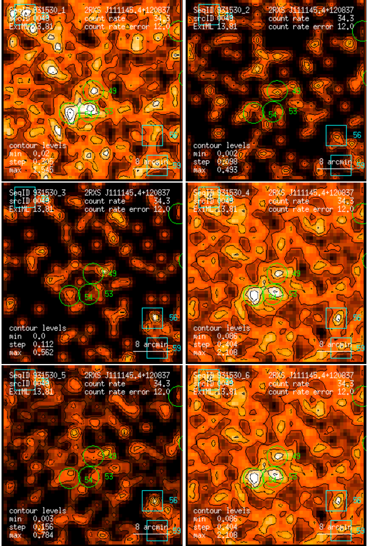
Figure 49: RASS 931530: detection 0049: band rate images, Gaussian filter: (1) PSPC channels 11 – 41, (2) 52 – 90, (3) 91 – 201, (4) 11 – 235, (5) 52 – 201, (6) 11 – 201. Broad band rates in counts/ks. Band rate contour levels in counts/ks/arcmin 2 .
