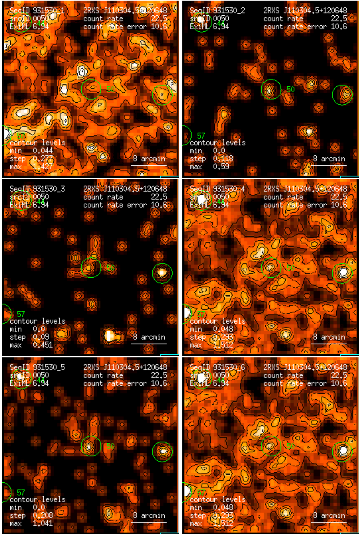
Figure 50: RASS 931530: detection 0050: band rate images, Gaussian filter: (1) PSPC channels 11 – 41, (2) 52 – 90, (3) 91 – 201, (4) 11 – 235, (5) 52 – 201, (6) 11 – 201. Broad band rates in counts/ks. Band rate contour levels in counts/ks/arcmin 2 .
