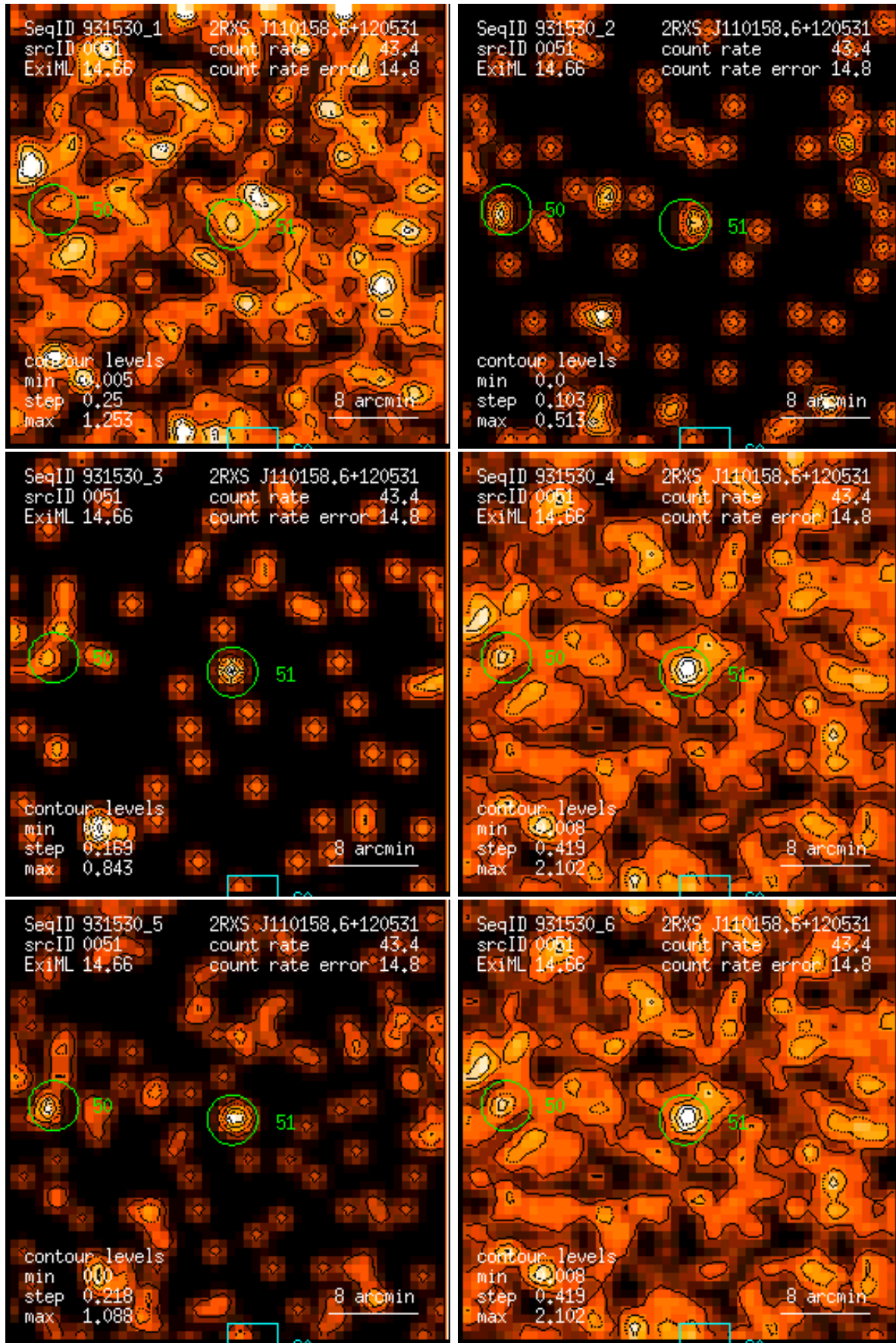
Figure 51: RASS 931530: detection 0051: band rate images, Gaussian filter: (1) PSPC channels 11 – 41, (2) 52 – 90, (3) 91 – 201, (4) 11 – 235, (5) 52 – 201, (6) 11 – 201. Broad band rates in counts/ks. Band rate contour levels in counts/ks/arcmin 2 .
