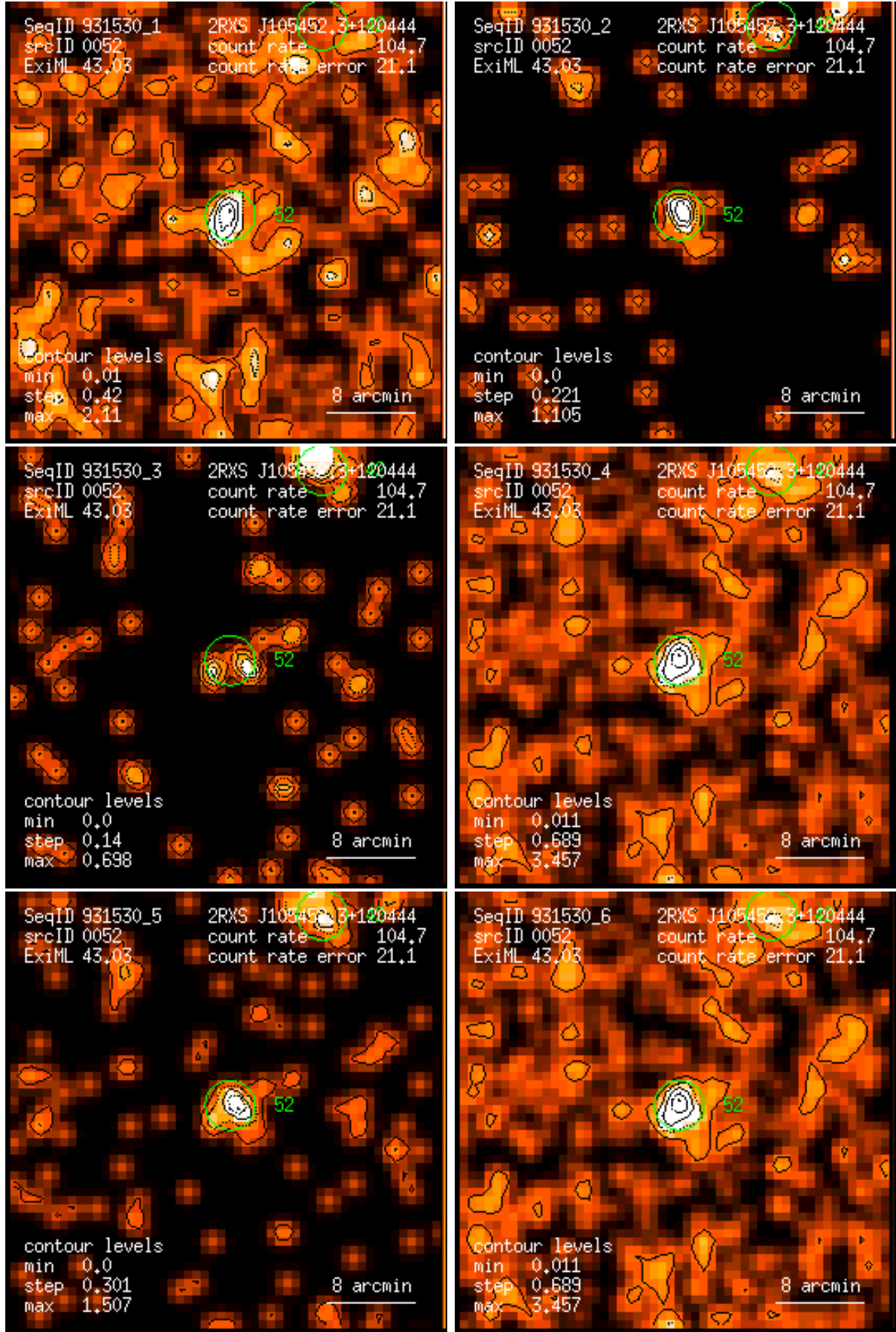
Figure 52: RASS 931530: detection 0052: band rate images, Gaussian filter: (1) PSPC channels 11 – 41, (2) 52 – 90, (3) 91 – 201, (4) 11 – 235, (5) 52 – 201, (6) 11 – 201. Broad band rates in counts/ks. Band rate contour levels in counts/ks/arcmin 2 .
