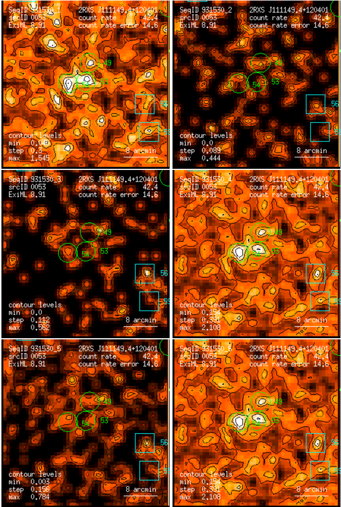
Figure 53: RASS 931530: detection 0053: band rate images, Gaussian filter: (1) PSPC channels 11 – 41, (2) 52 – 90, (3) 91 – 201, (4) 11 – 235, (5) 52 – 201, (6) 11 – 201. Broad band rates in counts/ks. Band rate contour levels in counts/ks/arcmin 2 .
