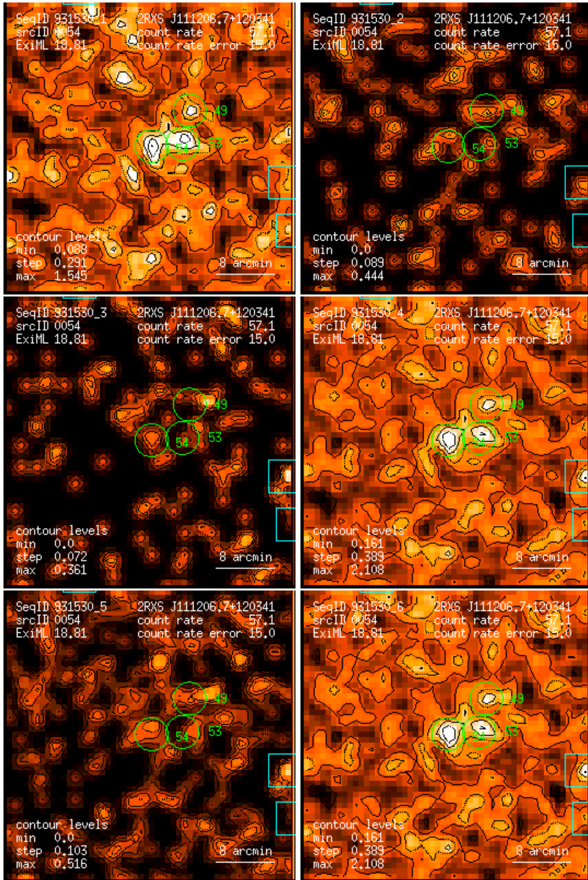
Figure 54: RASS 931530: detection 0054: band rate images, Gaussian filter: (1) PSPC channels 11 – 41, (2) 52 – 90, (3) 91 – 201, (4) 11 – 235, (5) 52 – 201, (6) 11 – 201. Broad band rates in counts/ks. Band rate contour levels in counts/ks/arcmin 2 .
