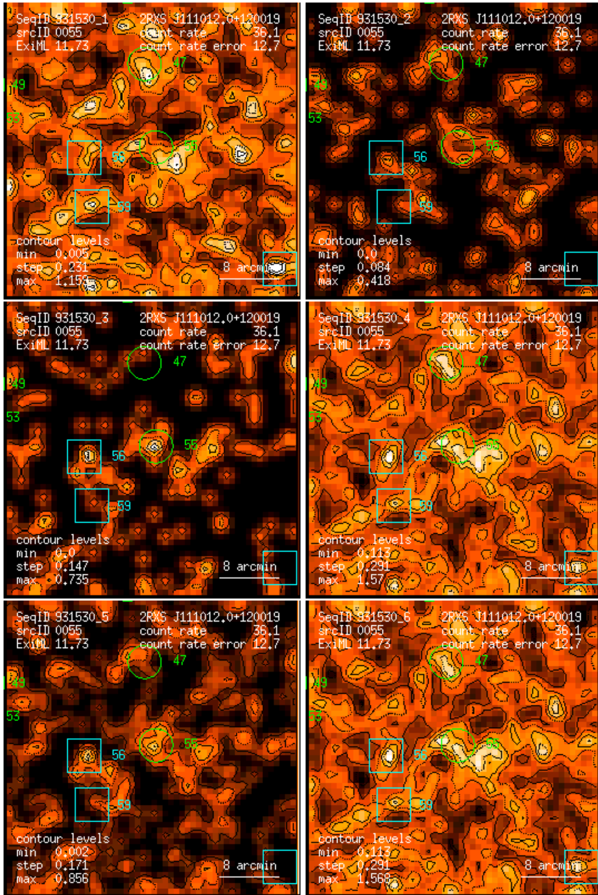
Figure 55: RASS 931530: detection 0055: band rate images, Gaussian filter: (1) PSPC channels 11 – 41, (2) 52 – 90, (3) 91 – 201, (4) 11 – 235, (5) 52 – 201, (6) 11 – 201. Broad band rates in counts/ks. Band rate contour levels in counts/ks/arcmin 2 .
