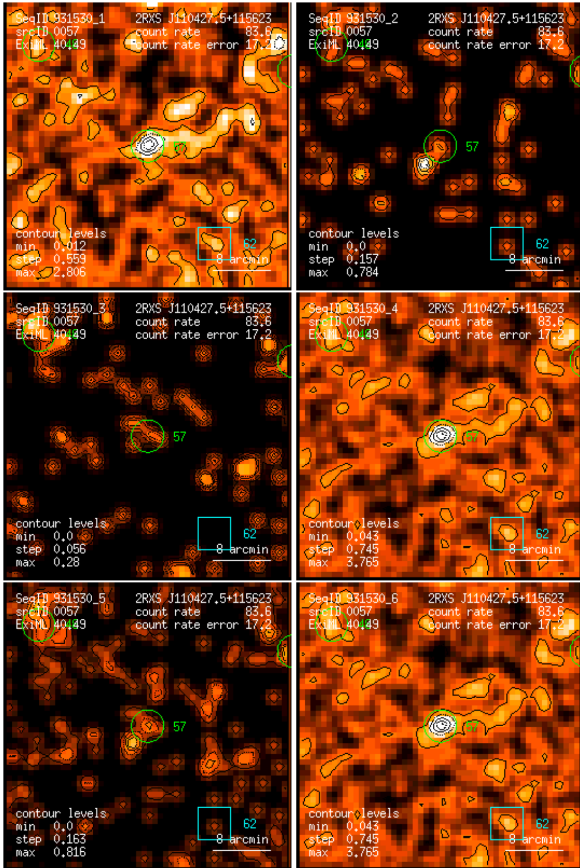
Figure 57: RASS 931530: detection 0057: band rate images, Gaussian filter: (1) PSPC channels 11 – 41, (2) 52 – 90, (3) 91 – 201, (4) 11 – 235, (5) 52 – 201, (6) 11 – 201. Broad band rates in counts/ks. Band rate contour levels in counts/ks/arcmin 2 .
