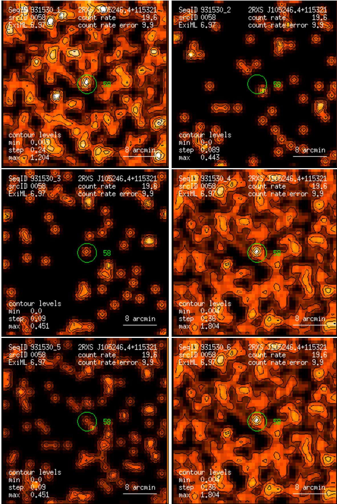
Figure 58: RASS 931530: detection 0058: band rate images, Gaussian filter: (1) PSPC channels 11 – 41, (2) 52 – 90, (3) 91 – 201, (4) 11 – 235, (5) 52 – 201, (6) 11 – 201. Broad band rates in counts/ks. Band rate contour levels in counts/ks/arcmin 2 .
