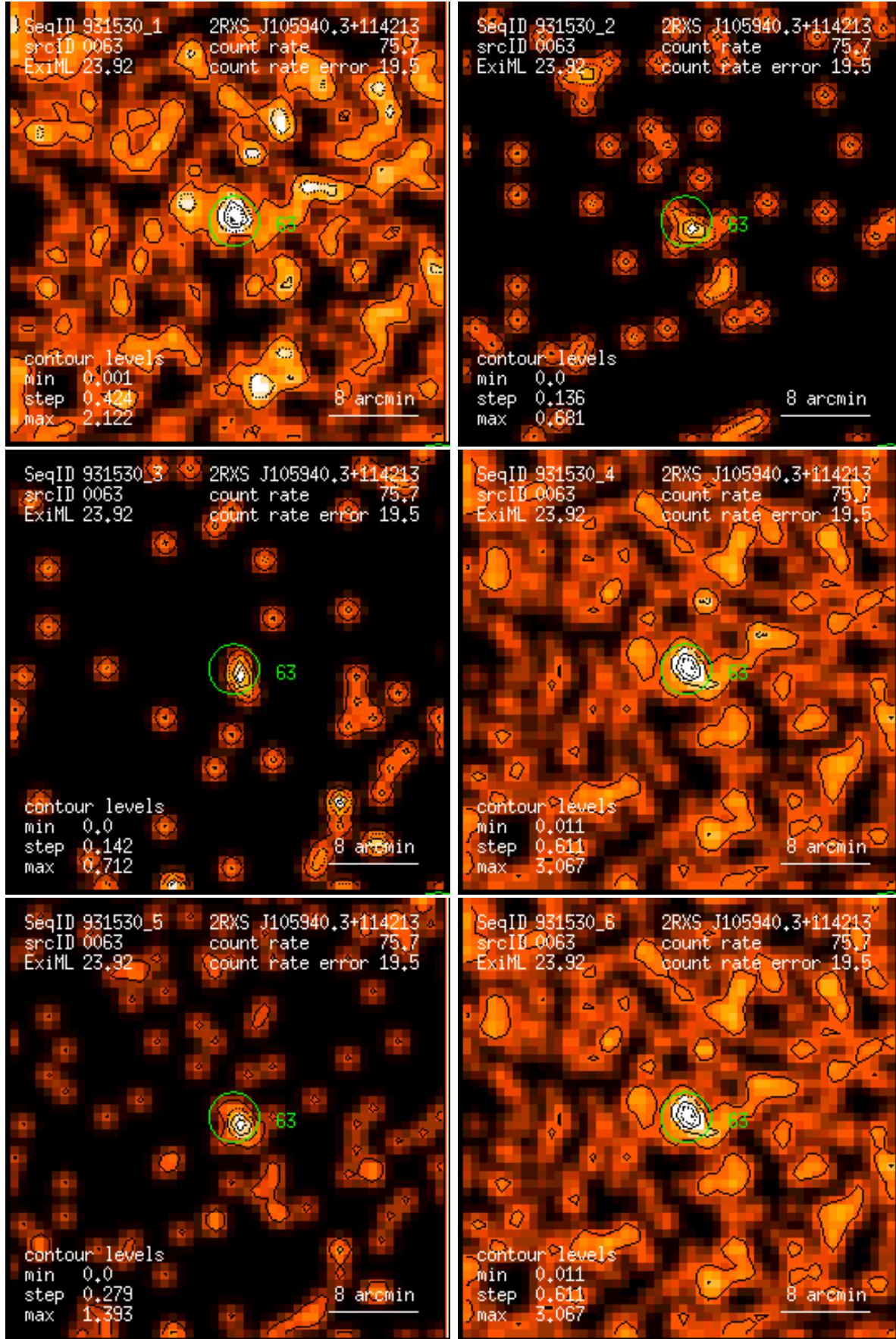
Figure 63: RASS 931530: detection 0063: band rate images, Gaussian filter: (1) PSPC channels 11 – 41, (2) 52 – 90, (3) 91 – 201, (4) 11 – 235, (5) 52 – 201, (6) 11 – 201. Broad band rates in counts/ks. Band rate contour levels in counts/ks/arcmin 2 .
