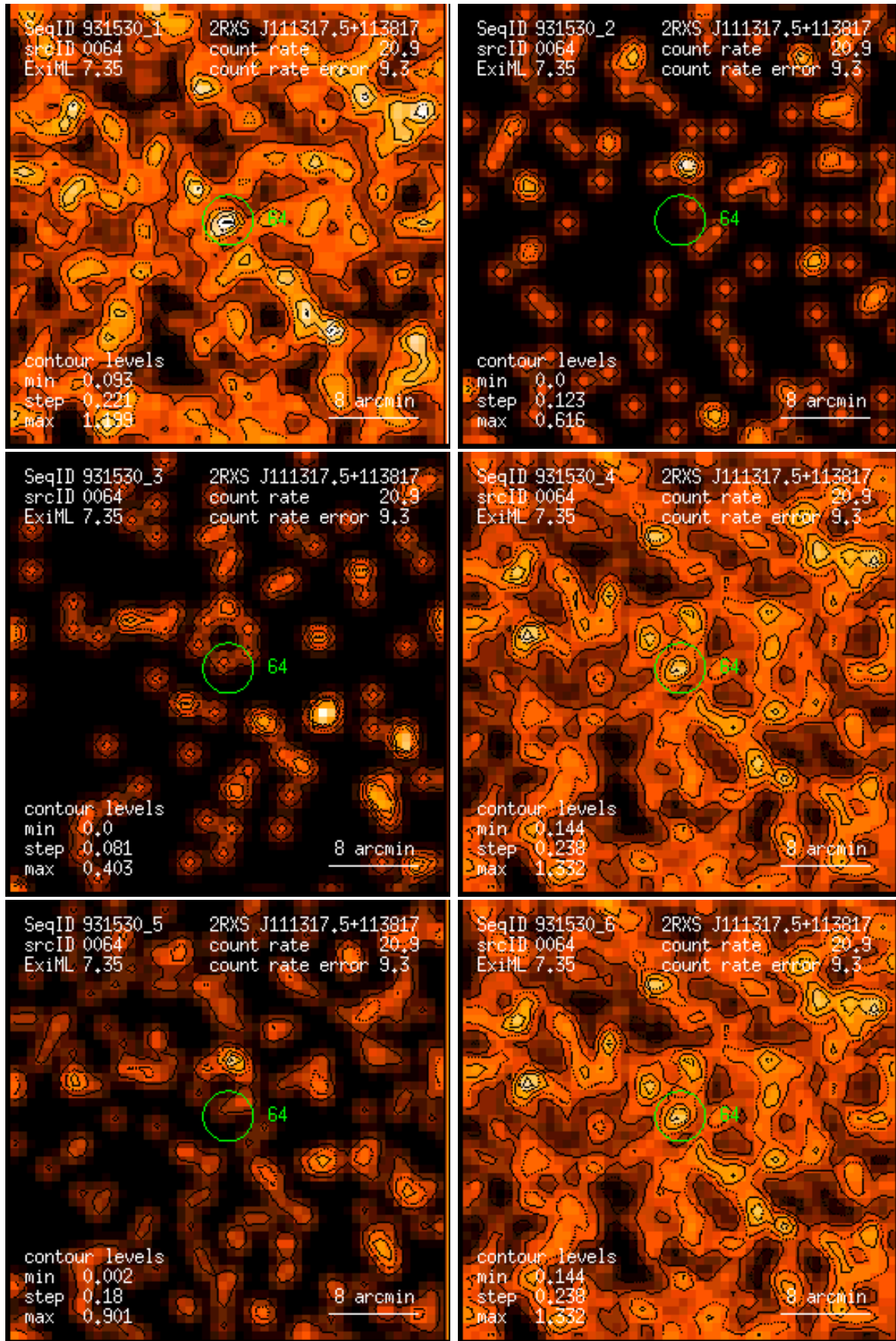
Figure 64: RASS 931530: detection 0064: band rate images, Gaussian filter: (1) PSPC channels 11 – 41, (2) 52 – 90, (3) 91 – 201, (4) 11 – 235, (5) 52 – 201, (6) 11 – 201. Broad band rates in counts/ks. Band rate contour levels in counts/ks/arcmin 2 .
