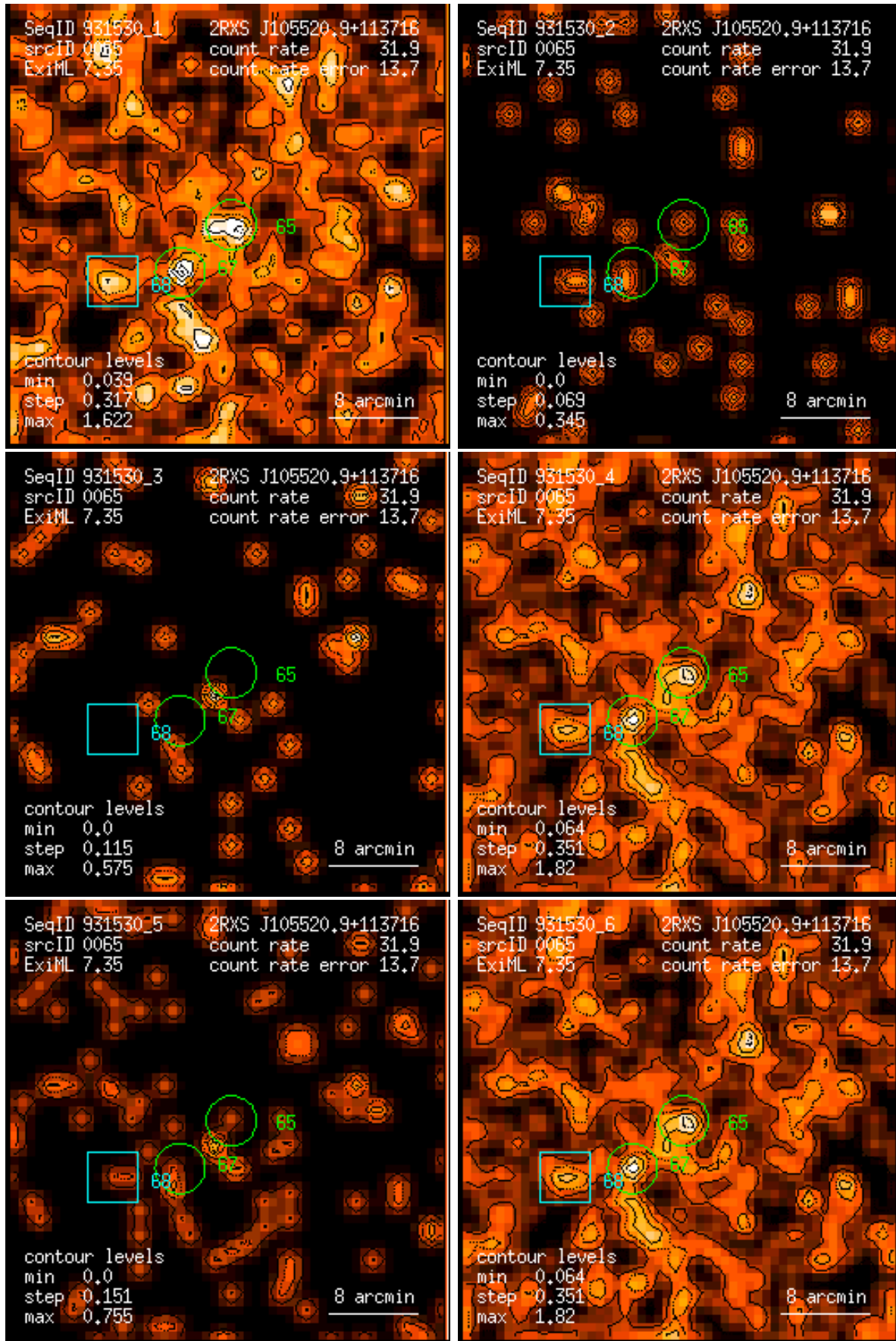
Figure 65: RASS 931530: detection 0065: band rate images, Gaussian filter: (1) PSPC channels 11 – 41, (2) 52 – 90, (3) 91 – 201, (4) 11 – 235, (5) 52 – 201, (6) 11 – 201. Broad band rates in counts/ks. Band rate contour levels in counts/ks/arcmin 2 .
