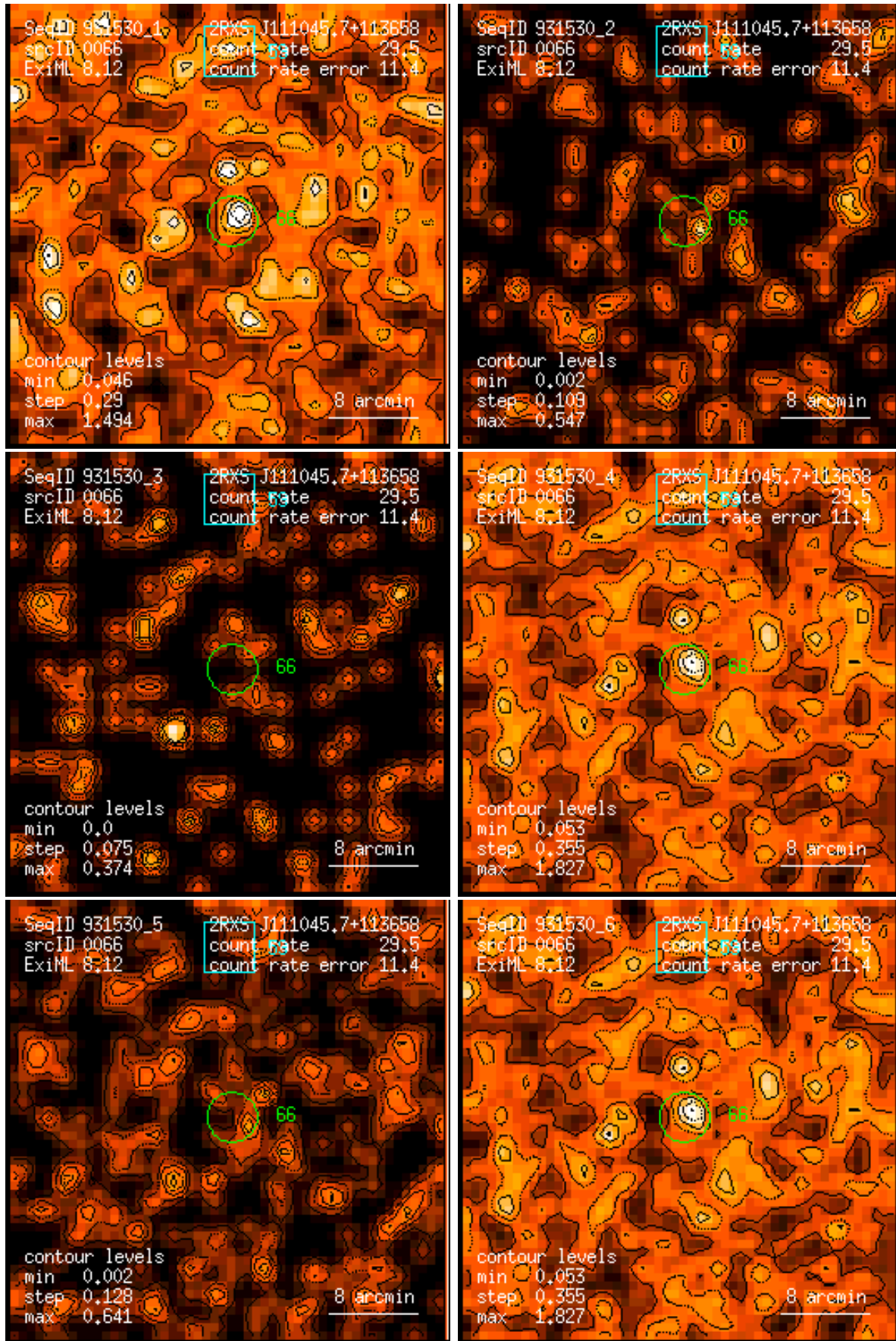
Figure 66: RASS 931530: detection 0066: band rate images, Gaussian filter: (1) PSPC channels 11 – 41, (2) 52 – 90, (3) 91 – 201, (4) 11 – 235, (5) 52 – 201, (6) 11 – 201. Broad band rates in counts/ks. Band rate contour levels in counts/ks/arcmin 2 .
