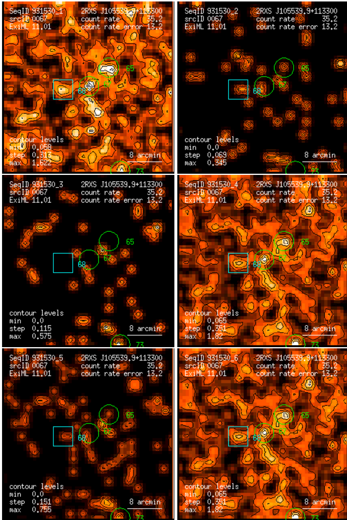
Figure 67: RASS 931530: detection 0067: band rate images, Gaussian filter: (1) PSPC channels 11 – 41, (2) 52 – 90, (3) 91 – 201, (4) 11 – 235, (5) 52 – 201, (6) 11 – 201. Broad band rates in counts/ks. Band rate contour levels in counts/ks/arcmin 2 .
