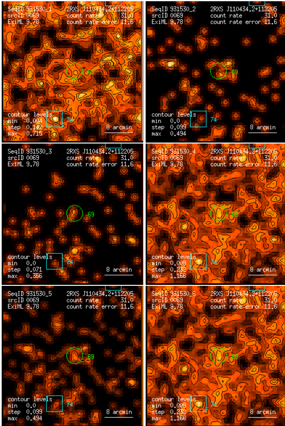
Figure 69: RASS 931530: detection 0069: band rate images, Gaussian filter: (1) PSPC channels 11 – 41, (2) 52 – 90, (3) 91 – 201, (4) 11 – 235, (5) 52 – 201, (6) 11 – 201. Broad band rates in counts/ks. Band rate contour levels in counts/ks/arcmin 2 .
