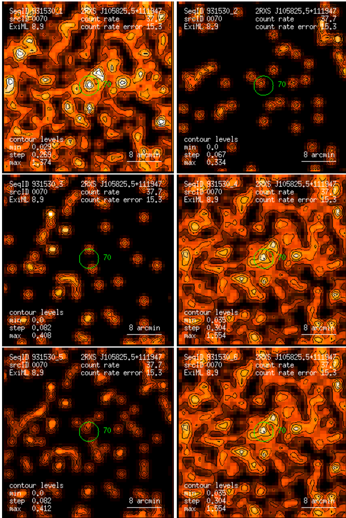
Figure 70: RASS 931530: detection 0070: band rate images, Gaussian filter: (1) PSPC channels 11 – 41, (2) 52 – 90, (3) 91 – 201, (4) 11 – 235, (5) 52 – 201, (6) 11 – 201. Broad band rates in counts/ks. Band rate contour levels in counts/ks/arcmin 2 .
