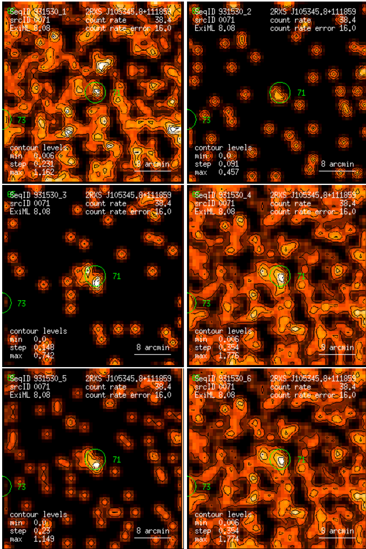
Figure 71: RASS 931530: detection 0071: band rate images, Gaussian filter: (1) PSPC channels 11 – 41, (2) 52 – 90, (3) 91 – 201, (4) 11 – 235, (5) 52 – 201, (6) 11 – 201. Broad band rates in counts/ks. Band rate contour levels in counts/ks/arcmin 2 .
