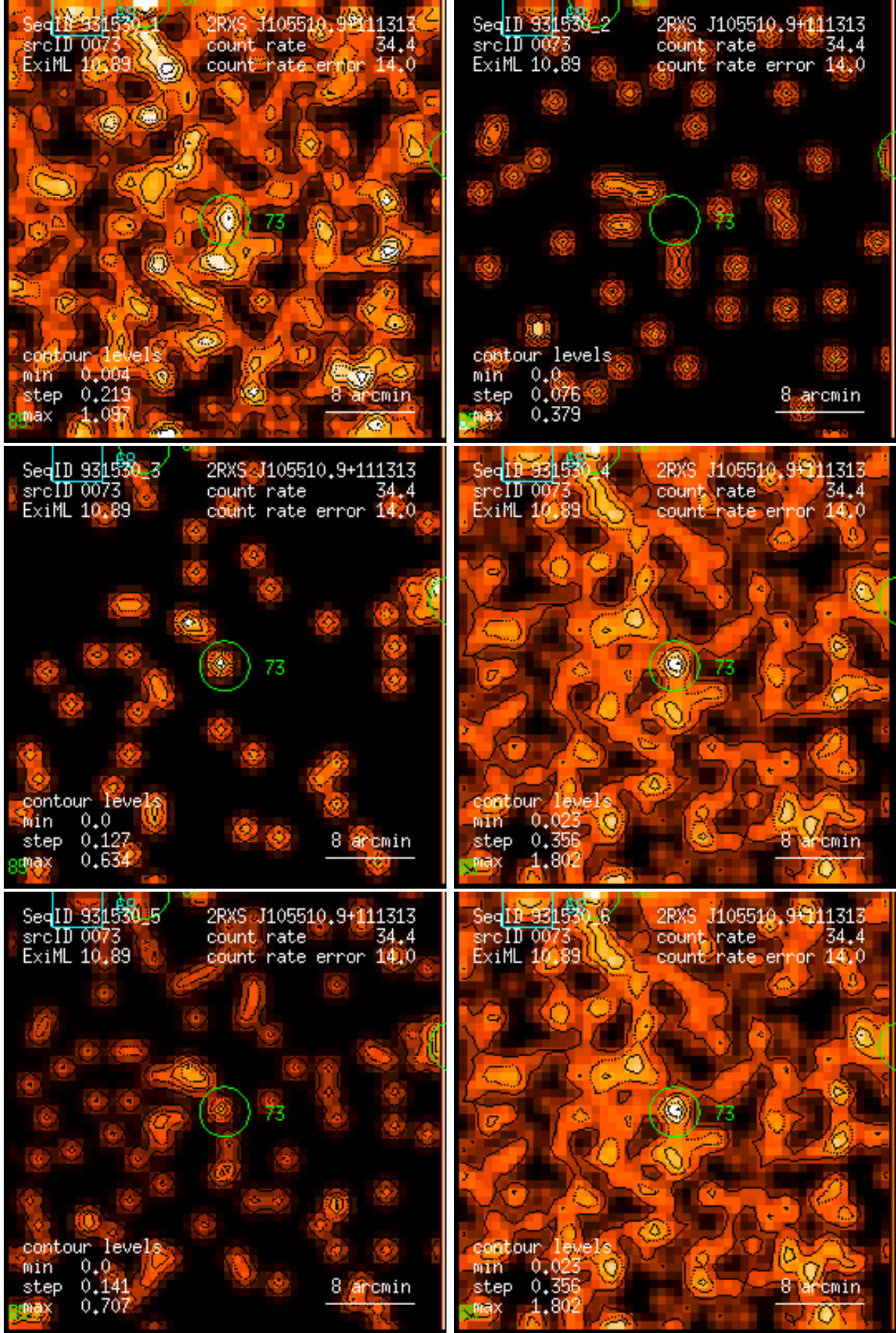
Figure 73: RASS 931530: detection 0073: band rate images, Gaussian filter: (1) PSPC channels 11 – 41, (2) 52 – 90, (3) 91 – 201, (4) 11 – 235, (5) 52 – 201, (6) 11 – 201. Broad band rates in counts/ks. Band rate contour levels in counts/ks/arcmin 2 .
