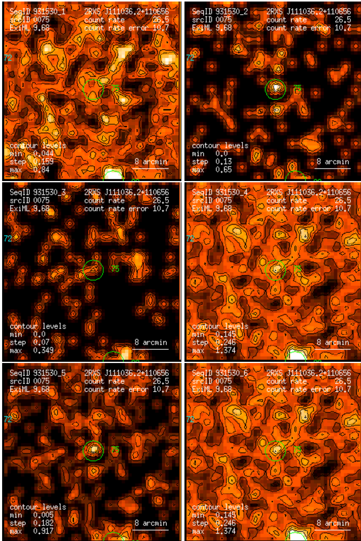
Figure 75: RASS 931530: detection 0075: band rate images, Gaussian filter: (1) PSPC channels 11 – 41, (2) 52 – 90, (3) 91 – 201, (4) 11 – 235, (5) 52 – 201, (6) 11 – 201. Broad band rates in counts/ks. Band rate contour levels in counts/ks/arcmin 2 .
