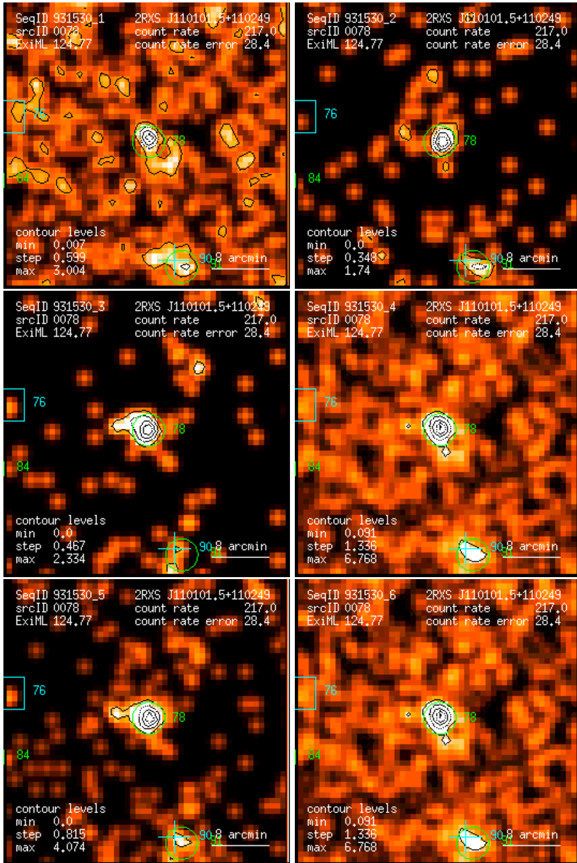
Figure 78: RASS 931530: detection 0078: band rate images, Gaussian filter: (1) PSPC channels 11 – 41, (2) 52 – 90, (3) 91 – 201, (4) 11 – 235, (5) 52 – 201, (6) 11 – 201. Broad band rates in counts/ks. Band rate contour levels in counts/ks/arcmin 2 .
