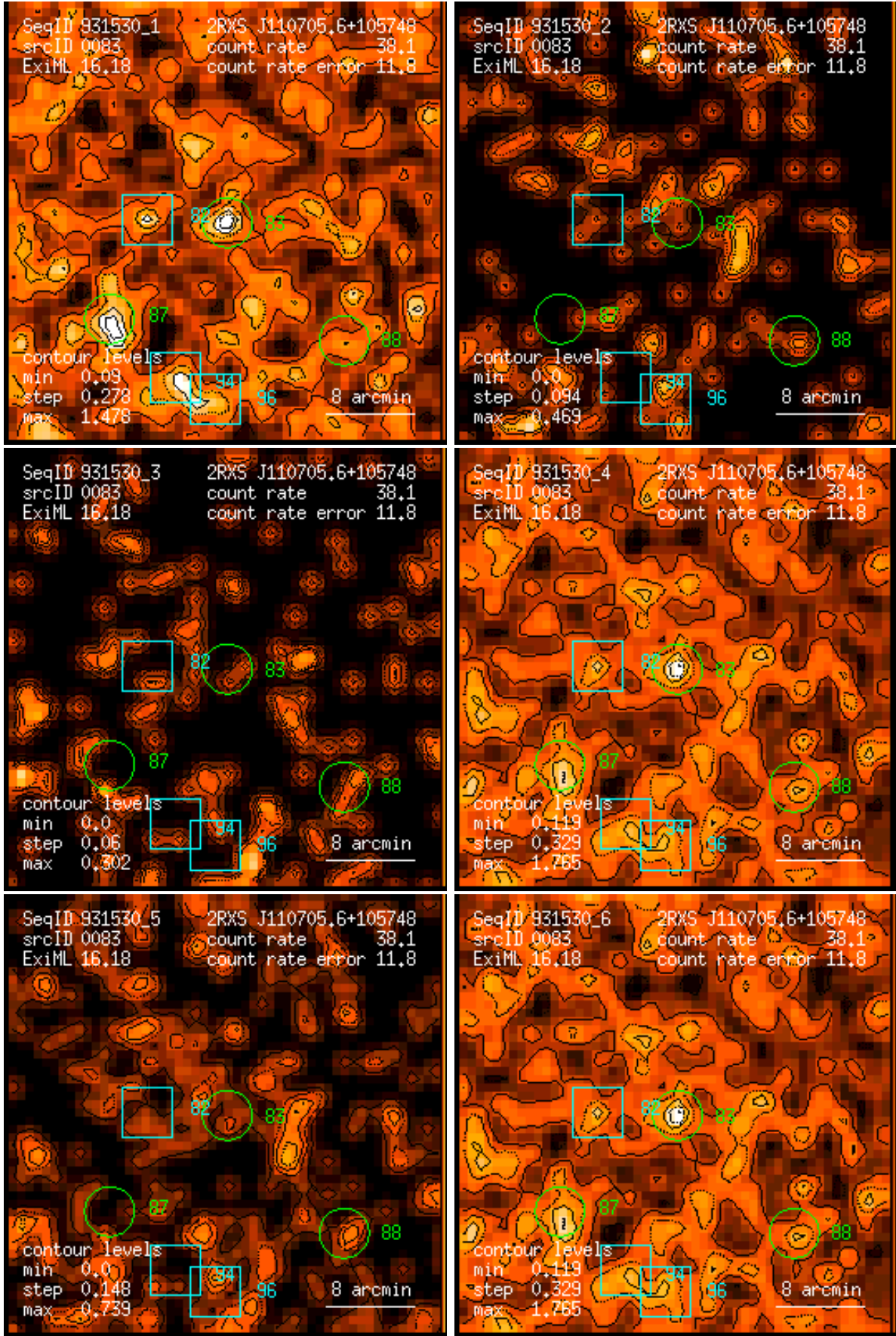
Figure 83: RASS 931530: detection 0083: band rate images, Gaussian filter: (1) PSPC channels 11 – 41, (2) 52 – 90, (3) 91 – 201, (4) 11 – 235, (5) 52 – 201, (6) 11 – 201. Broad band rates in counts/ks. Band rate contour levels in counts/ks/arcmin 2 .
