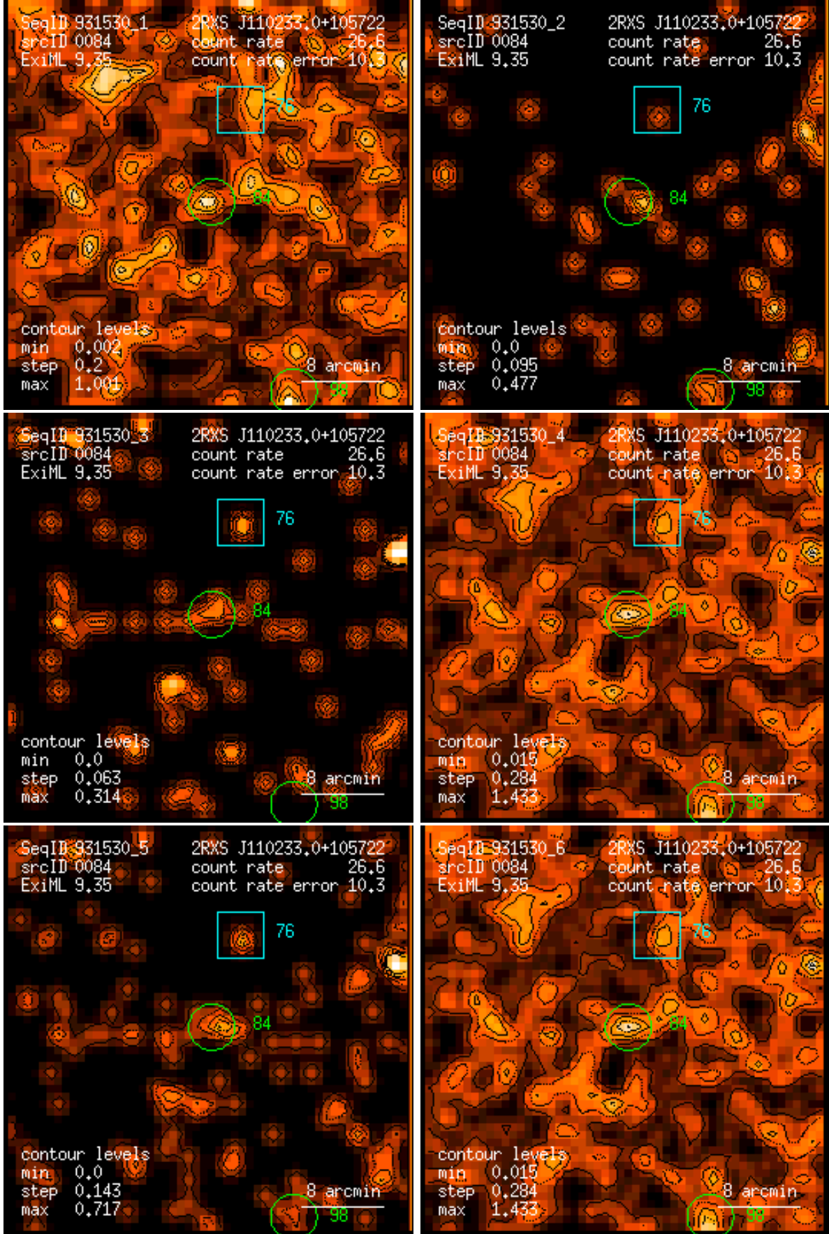
Figure 84: RASS 931530: detection 0084: band rate images, Gaussian filter: (1) PSPC channels 11 – 41, (2) 52 – 90, (3) 91 – 201, (4) 11 – 235, (5) 52 – 201, (6) 11 – 201. Broad band rates in counts/ks. Band rate contour levels in counts/ks/arcmin 2 .
