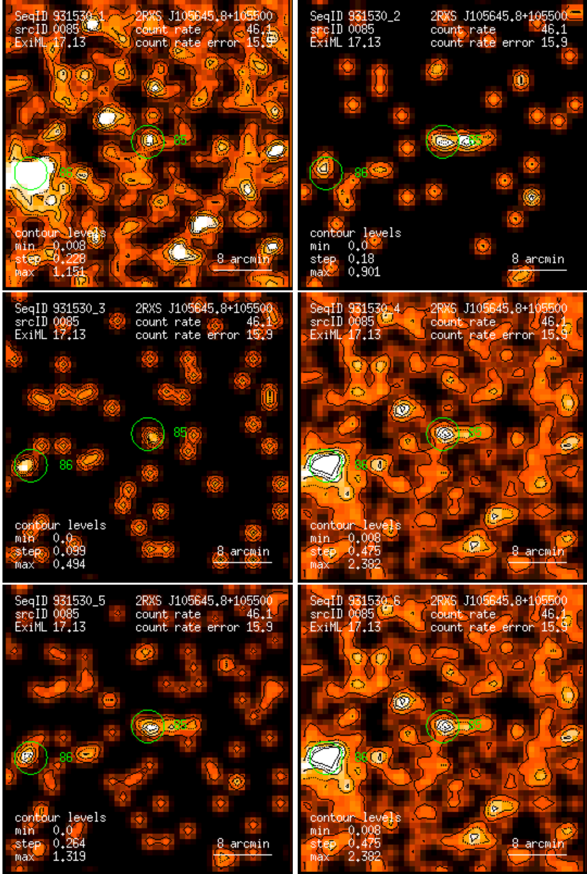
Figure 85: RASS 931530: detection 0085: band rate images, Gaussian filter: (1) PSPC channels 11 – 41, (2) 52 – 90, (3) 91 – 201, (4) 11 – 235, (5) 52 – 201, (6) 11 – 201. Broad band rates in counts/ks. Band rate contour levels in counts/ks/arcmin 2 .
