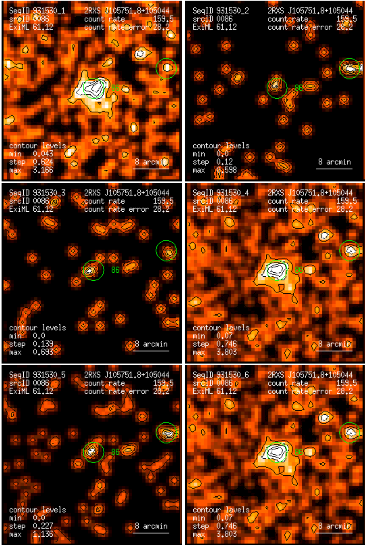
Figure 86: RASS 931530: detection 0086: band rate images, Gaussian filter: (1) PSPC channels 11 – 41, (2) 52 – 90, (3) 91 – 201, (4) 11 – 235, (5) 52 – 201, (6) 11 – 201. Broad band rates in counts/ks. Band rate contour levels in counts/ks/arcmin 2 .
