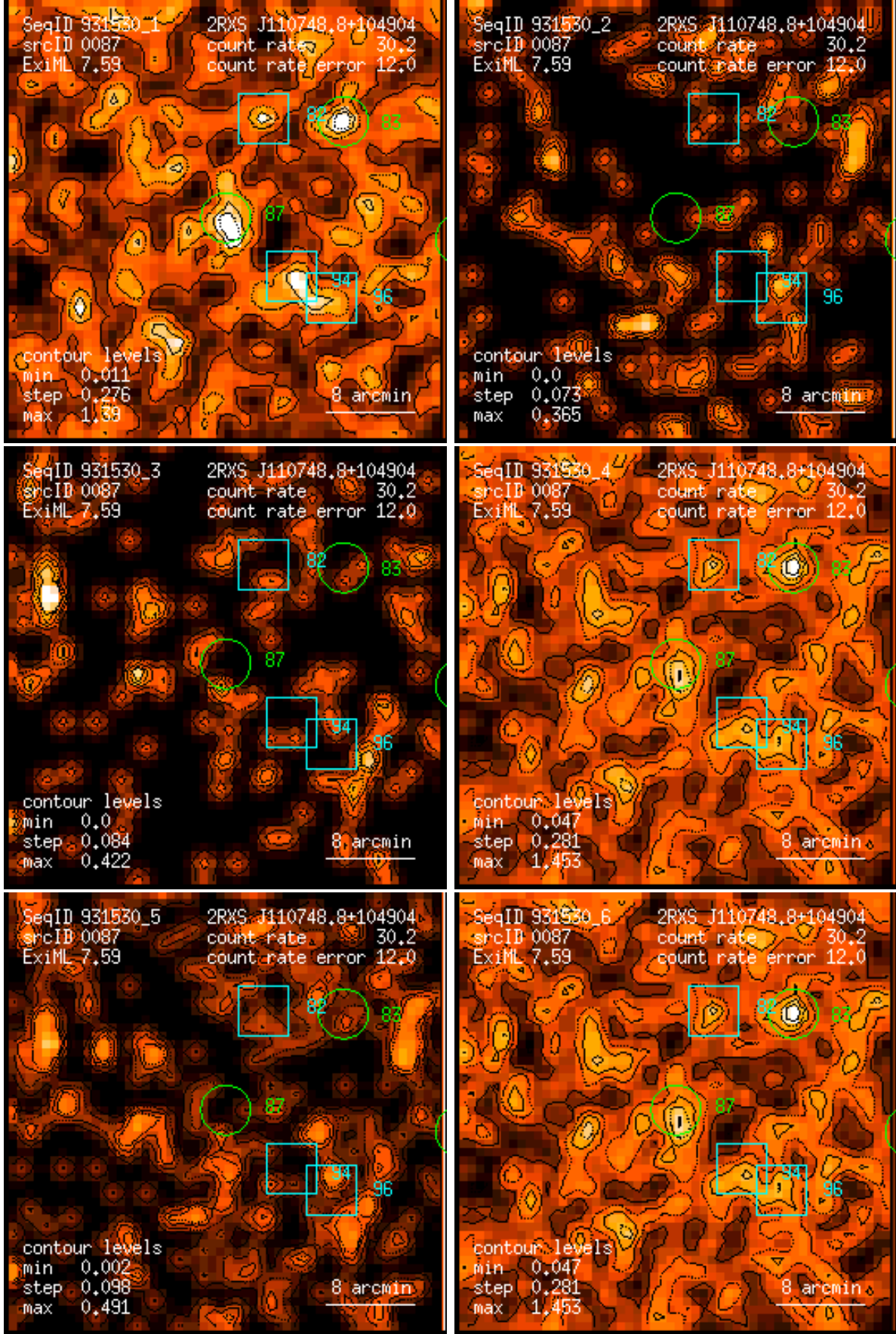
Figure 87: RASS 931530: detection 0087: band rate images, Gaussian filter: (1) PSPC channels 11 – 41, (2) 52 – 90, (3) 91 – 201, (4) 11 – 235, (5) 52 – 201, (6) 11 – 201. Broad band rates in counts/ks. Band rate contour levels in counts/ks/arcmin 2 .
