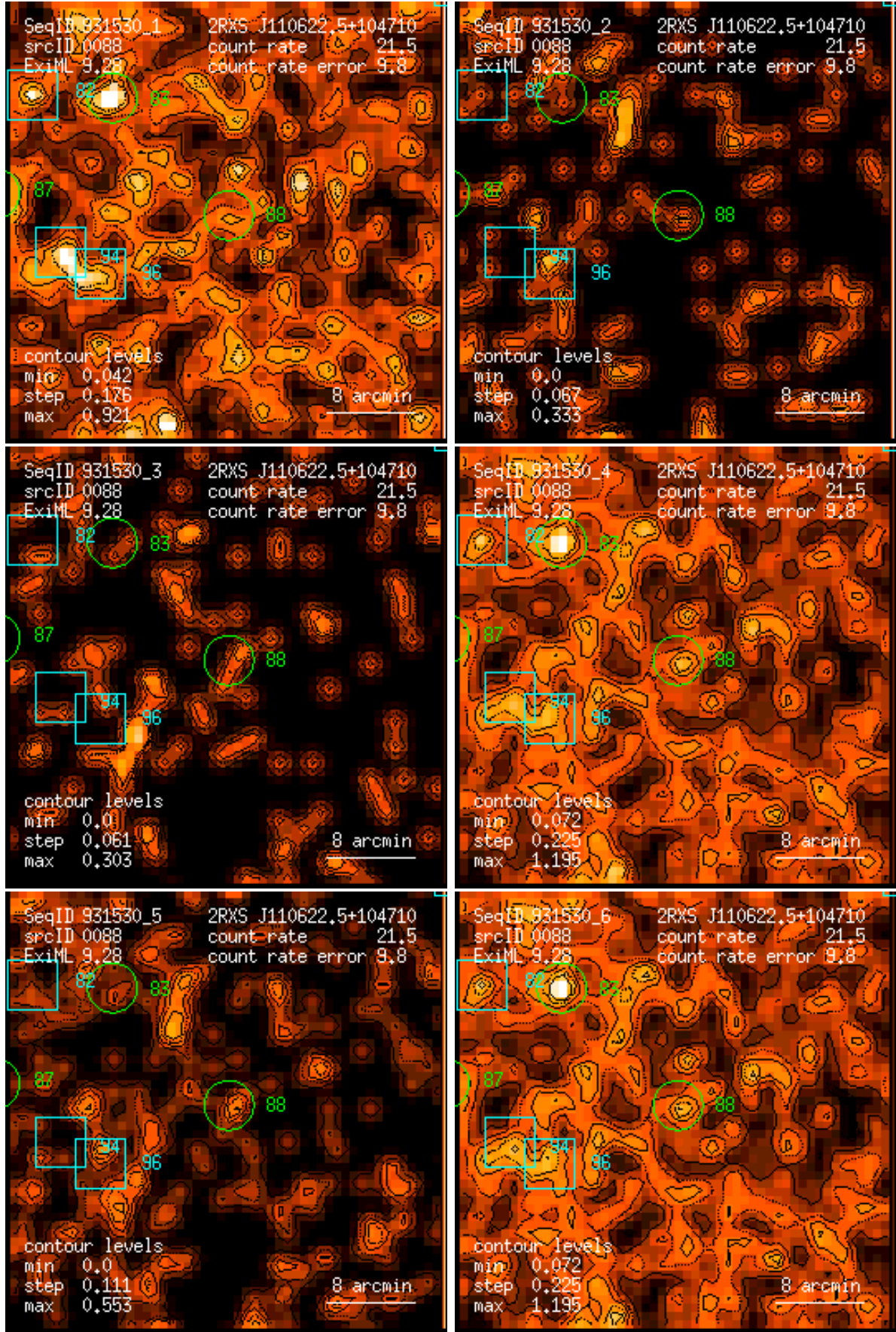
Figure 88: RASS 931530: detection 0088: band rate images, Gaussian filter: (1) PSPC channels 11 – 41, (2) 52 – 90, (3) 91 – 201, (4) 11 – 235, (5) 52 – 201, (6) 11 – 201. Broad band rates in counts/ks. Band rate contour levels in counts/ks/arcmin 2 .
