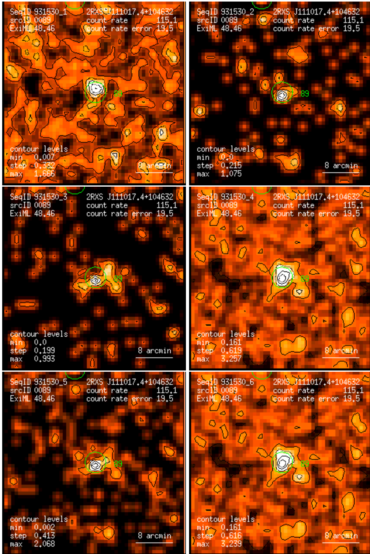
Figure 89: RASS 931530: detection 0089: band rate images, Gaussian filter: (1) PSPC channels 11 – 41, (2) 52 – 90, (3) 91 – 201, (4) 11 – 235, (5) 52 – 201, (6) 11 – 201. Broad band rates in counts/ks. Band rate contour levels in counts/ks/arcmin 2 .
