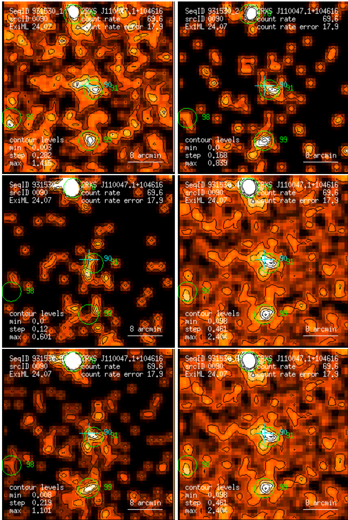
Figure 90: RASS 931530: detection 0090: band rate images, Gaussian filter: (1) PSPC channels 11 – 41, (2) 52 – 90, (3) 91 – 201, (4) 11 – 235, (5) 52 – 201, (6) 11 – 201. Broad band rates in counts/ks. Band rate contour levels in counts/ks/arcmin 2 .
