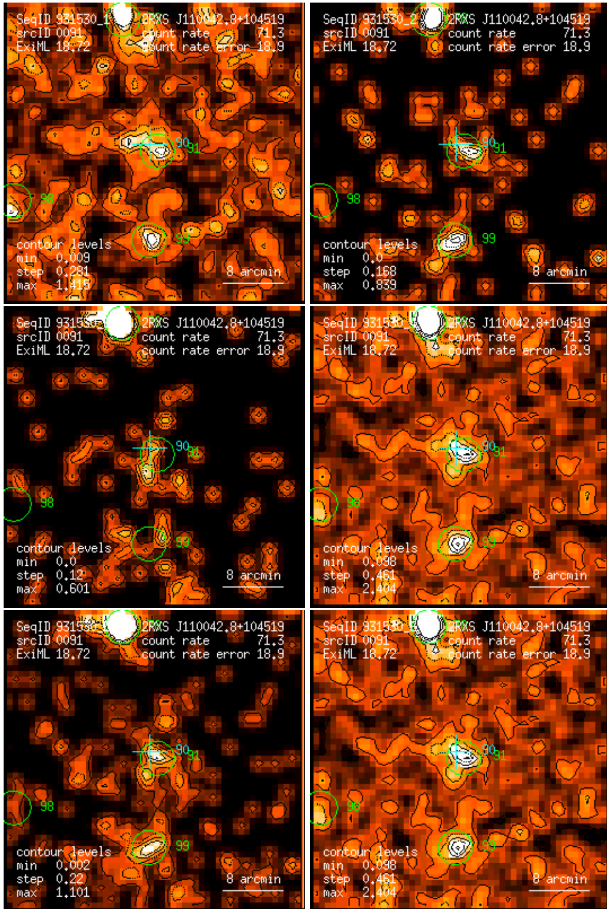
Figure 91: RASS 931530: detection 0091: band rate images, Gaussian filter: (1) PSPC channels 11 – 41, (2) 52 – 90, (3) 91 – 201, (4) 11 – 235, (5) 52 – 201, (6) 11 – 201. Broad band rates in counts/ks. Band rate contour levels in counts/ks/arcmin 2 .
