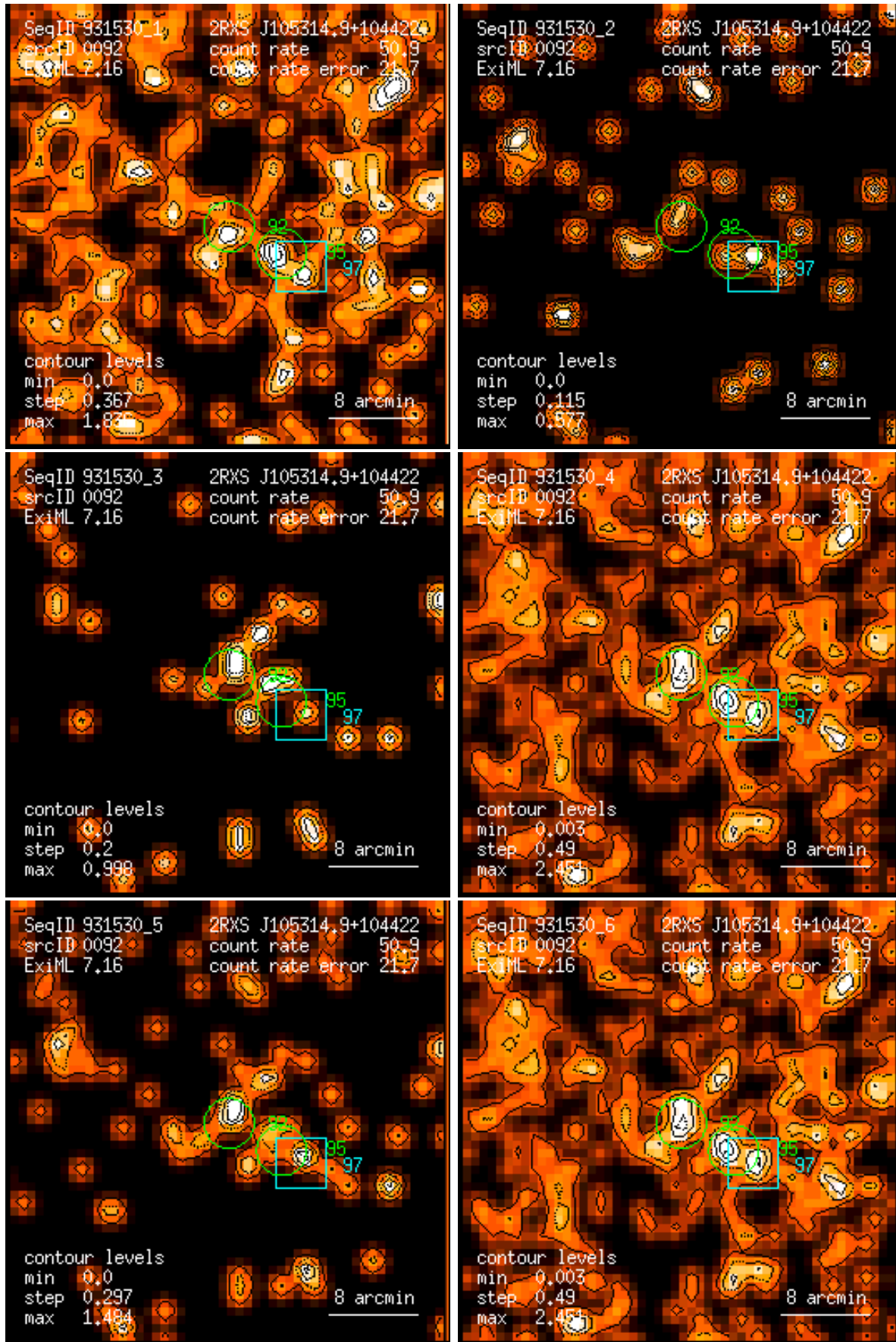
Figure 92: RASS 931530: detection 0092: band rate images, Gaussian filter: (1) PSPC channels 11 – 41, (2) 52 – 90, (3) 91 – 201, (4) 11 – 235, (5) 52 – 201, (6) 11 – 201. Broad band rates in counts/ks. Band rate contour levels in counts/ks/arcmin 2 .
