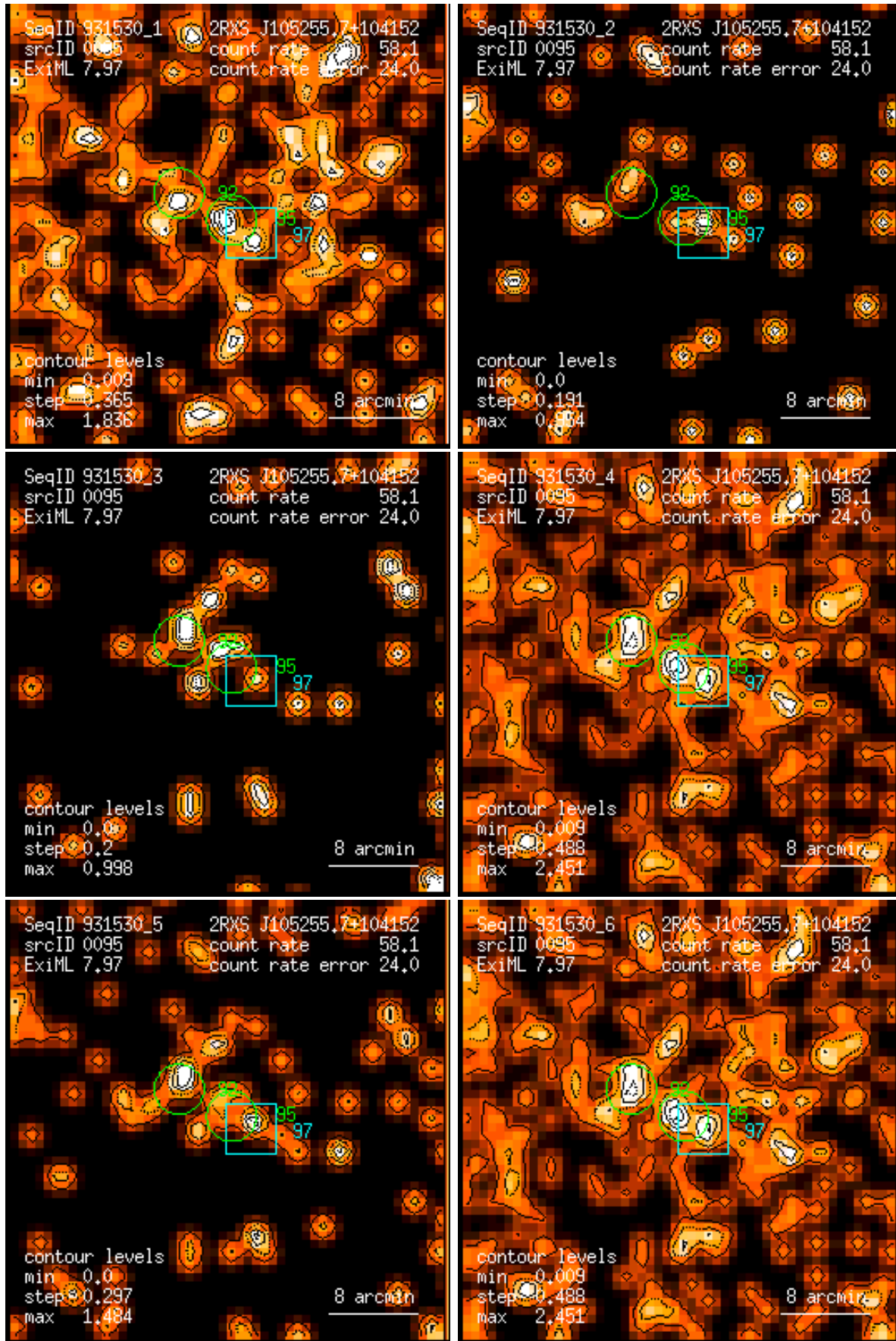
Figure 95: RASS 931530: detection 0095: band rate images, Gaussian filter: (1) PSPC channels 11 – 41, (2) 52 – 90, (3) 91 – 201, (4) 11 – 235, (5) 52 – 201, (6) 11 – 201. Broad band rates in counts/ks. Band rate contour levels in counts/ks/arcmin 2 .
