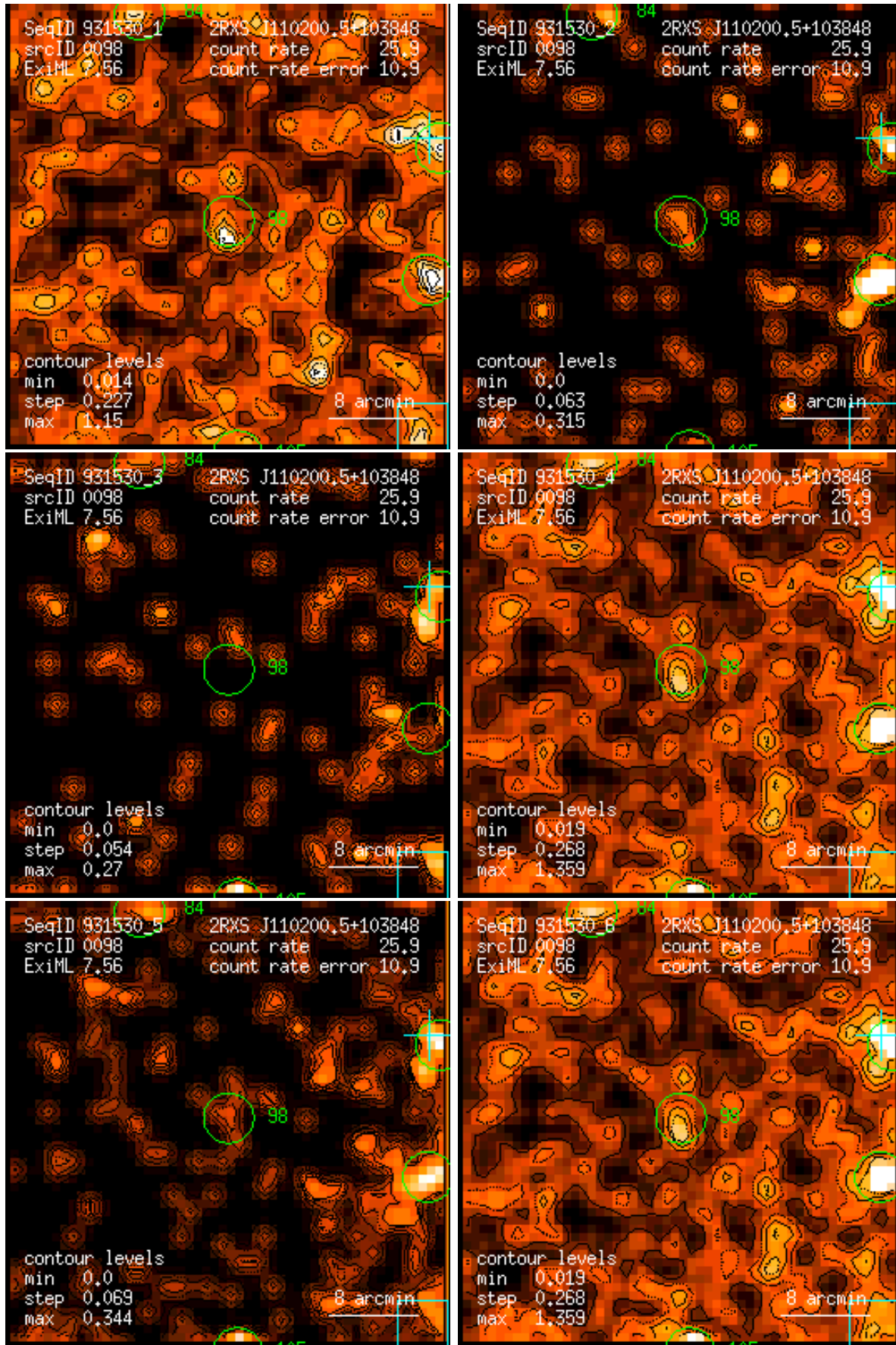
Figure 98: RASS 931530: detection 0098: band rate images, Gaussian filter: (1) PSPC channels 11 – 41, (2) 52 – 90, (3) 91 – 201, (4) 11 – 235, (5) 52 – 201, (6) 11 – 201. Broad band rates in counts/ks. Band rate contour levels in counts/ks/arcmin 2 .
