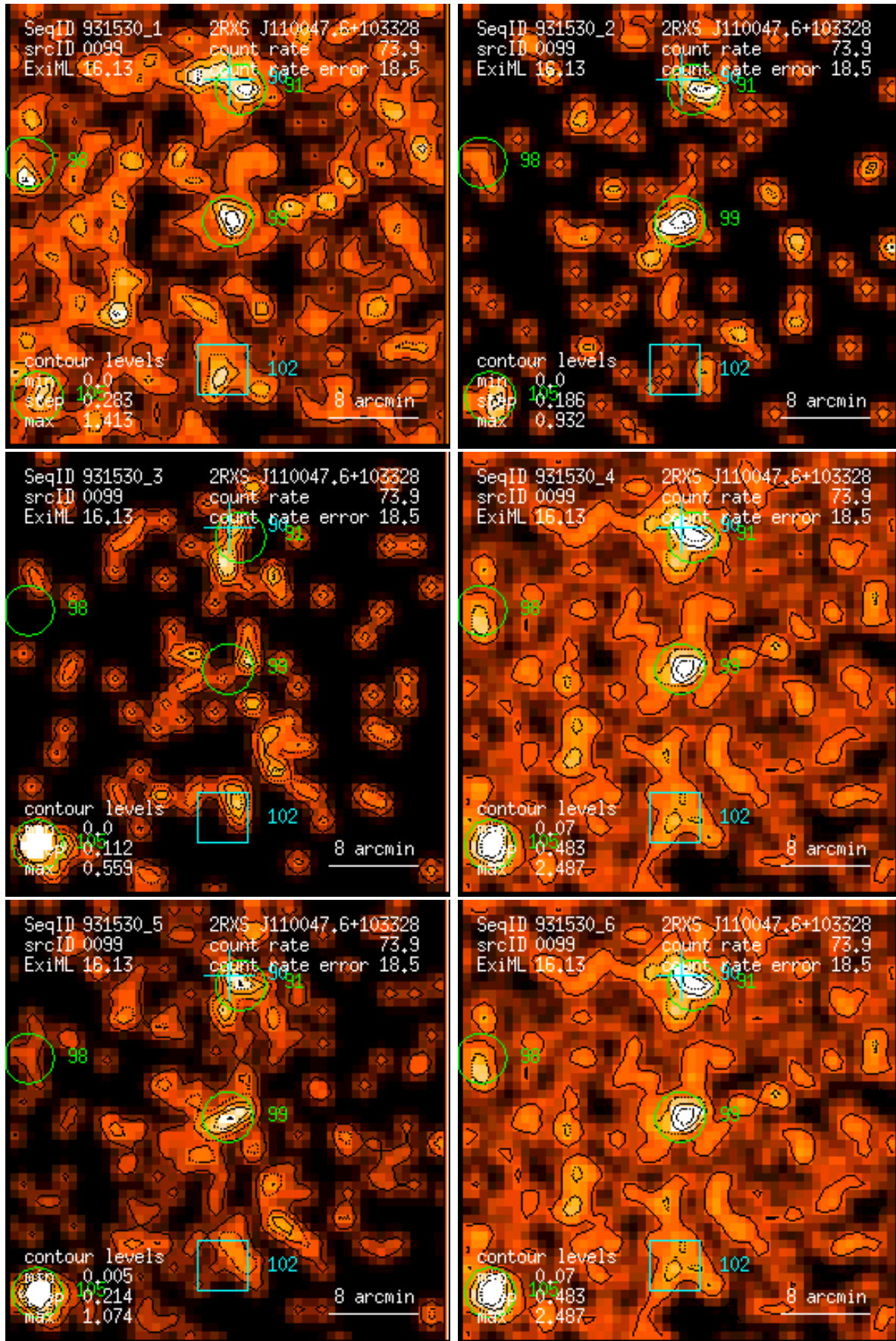
Figure 99: RASS 931530: detection 0099: band rate images, Gaussian filter: (1) PSPC channels 11 – 41, (2) 52 – 90, (3) 91 – 201, (4) 11 – 235, (5) 52 – 201, (6) 11 – 201. Broad band rates in counts/ks. Band rate contour levels in counts/ks/arcmin 2 .
