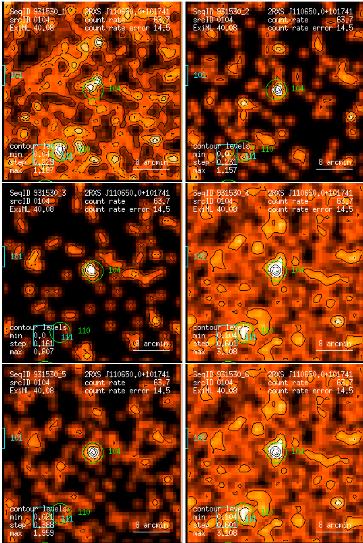
Figure 104: RASS 931530: detection 0104: band rate images, Gaussian filter: (1) PSPC channels 11 – 41, (2) 52 – 90, (3) 91 – 201, (4) 11 – 235, (5) 52 – 201, (6) 11 – 201. Broad band rates in counts/ks. Band rate contour levels in counts/ks/arcmin 2 .
