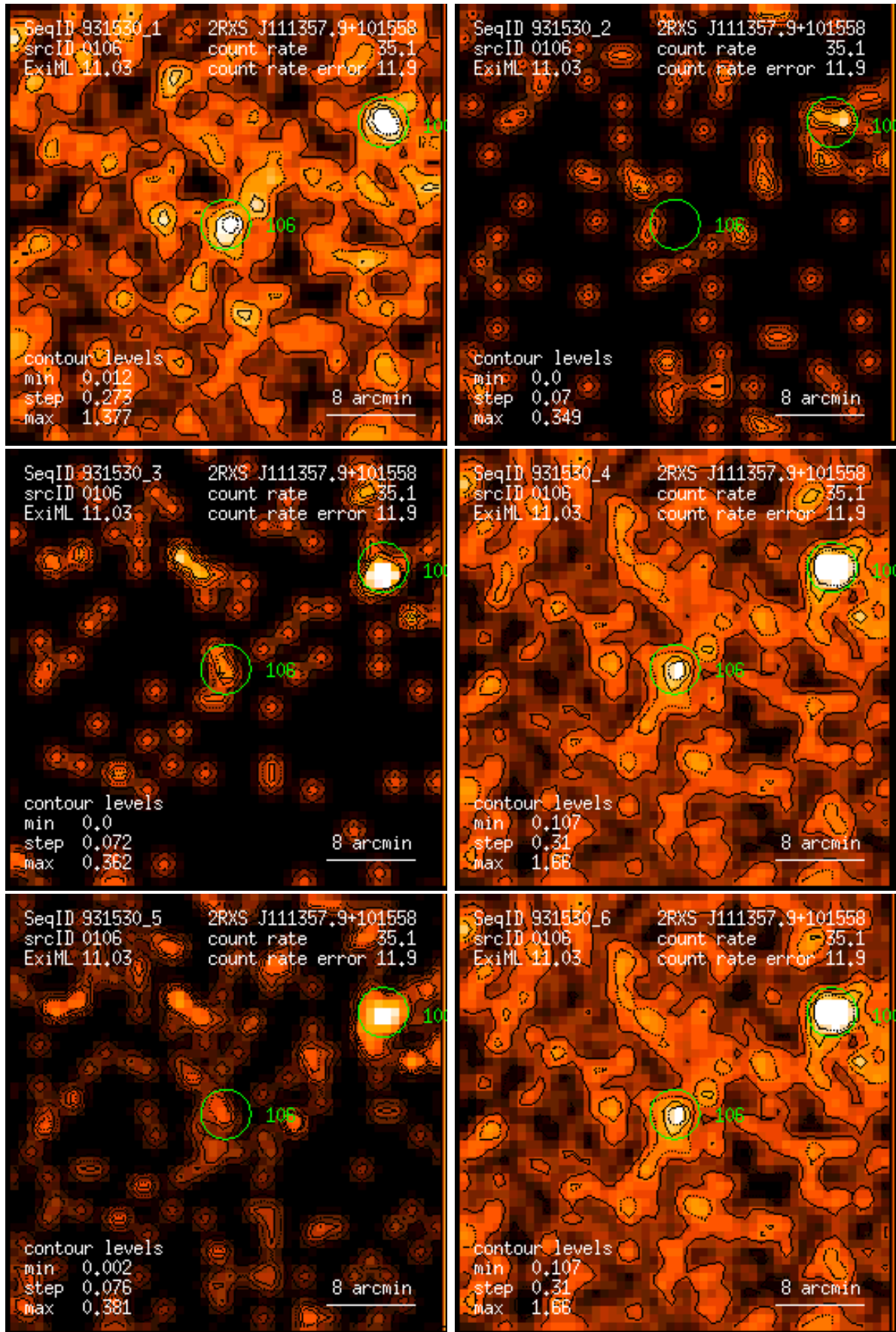
Figure 106: RASS 931530: detection 0106: band rate images, Gaussian filter: (1) PSPC channels 11 – 41, (2) 52 – 90, (3) 91 – 201, (4) 11 – 235, (5) 52 – 201, (6) 11 – 201. Broad band rates in counts/ks. Band rate contour levels in counts/ks/arcmin 2 .
