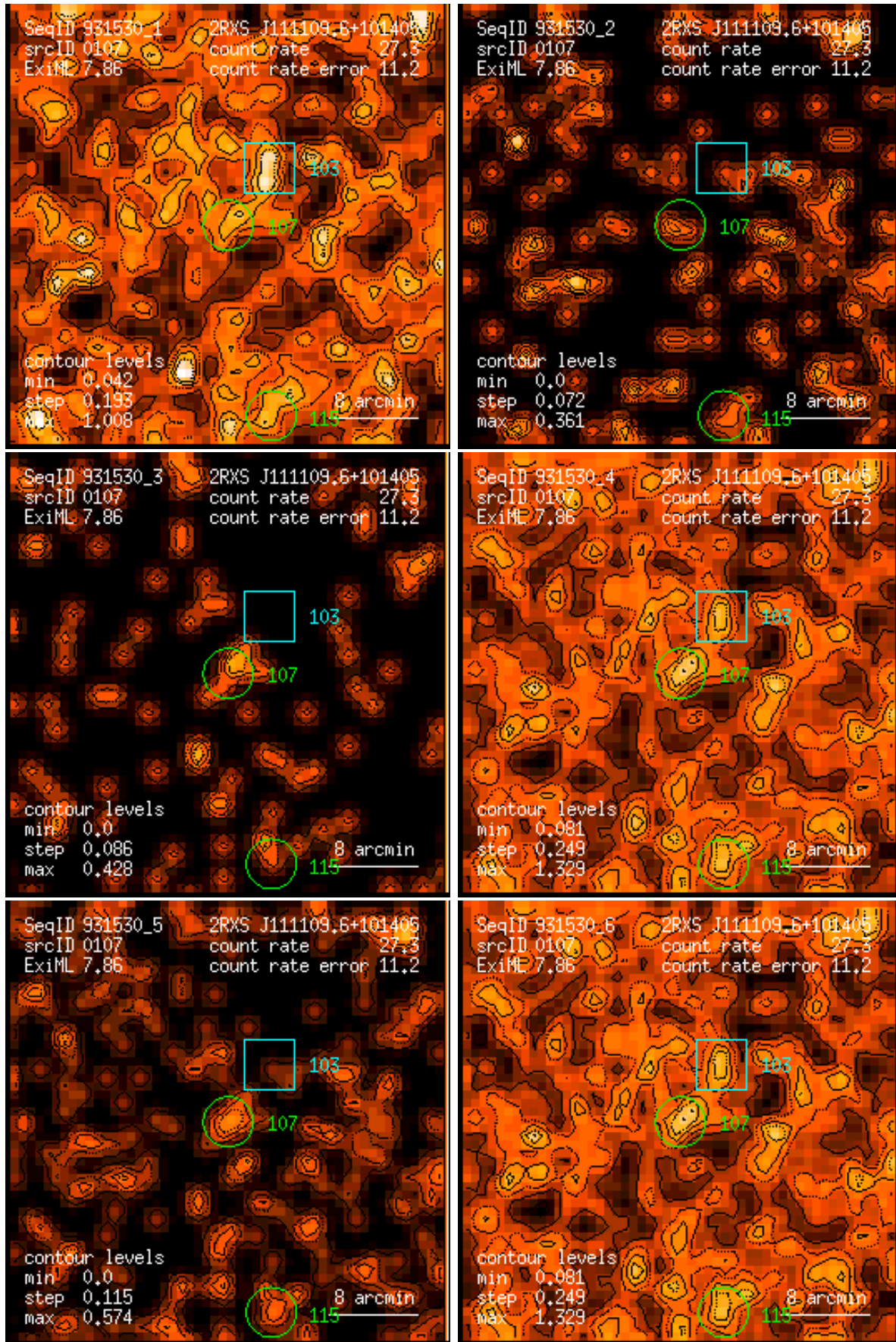
Figure 107: RASS 931530: detection 0107: band rate images, Gaussian filter: (1) PSPC channels 11 – 41, (2) 52 – 90, (3) 91 – 201, (4) 11 – 235, (5) 52 – 201, (6) 11 – 201. Broad band rates in counts/ks. Band rate contour levels in counts/ks/arcmin 2 .
