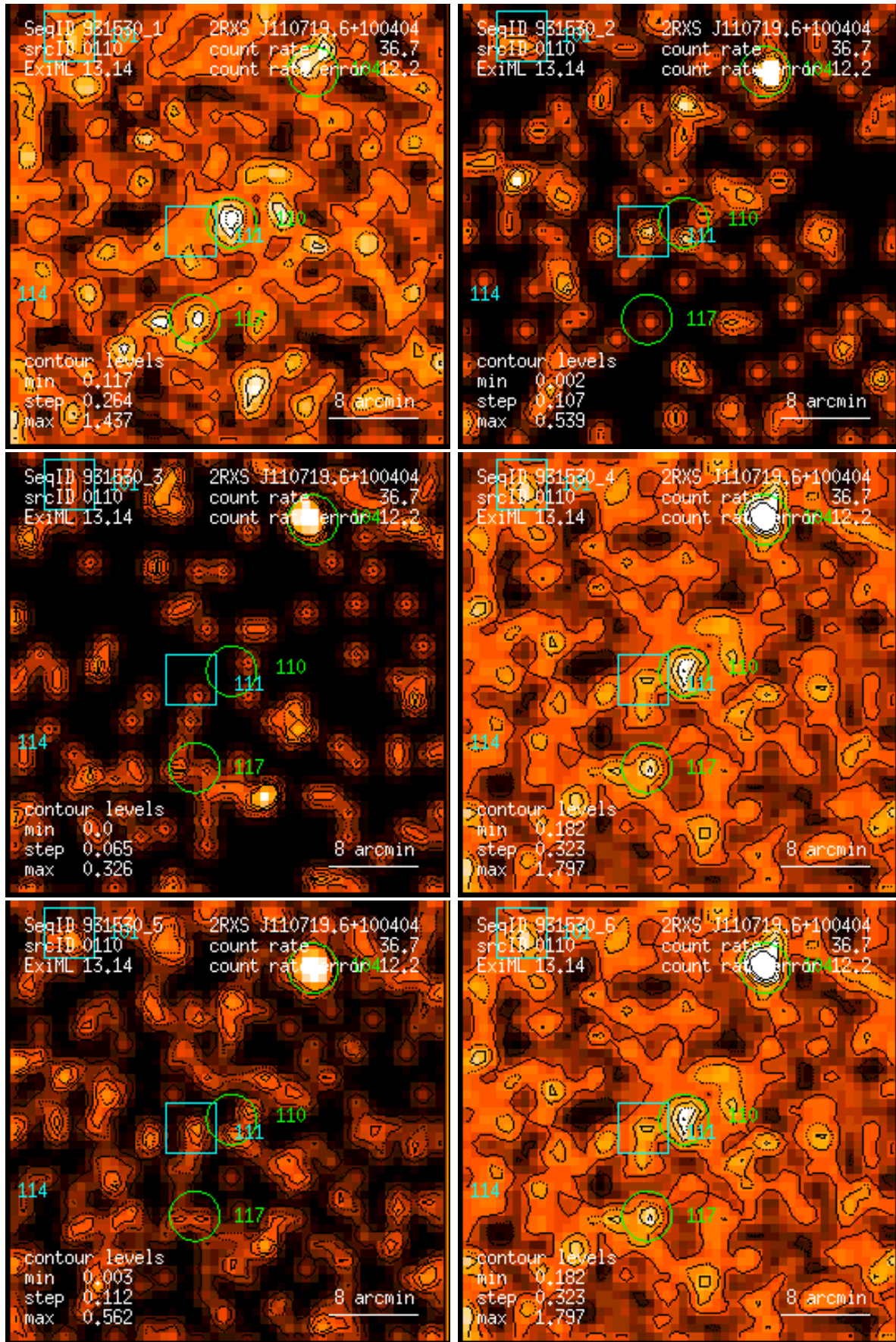
Figure 110: RASS 931530: detection 0110: band rate images, Gaussian filter: (1) PSPC channels 11 – 41, (2) 52 – 90, (3) 91 – 201, (4) 11 – 235, (5) 52 – 201, (6) 11 – 201. Broad band rates in counts/ks. Band rate contour levels in counts/ks/arcmin 2 .
