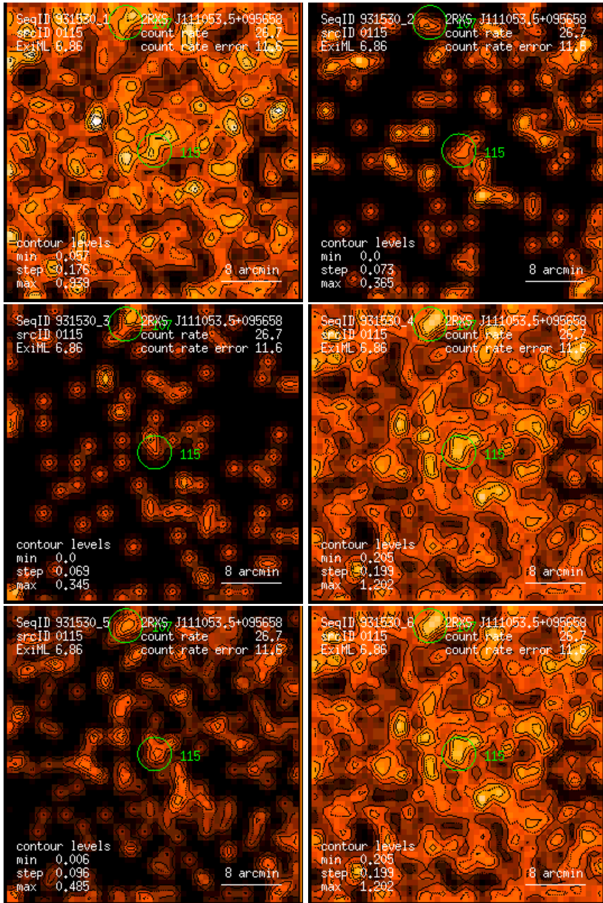
Figure 115: RASS 931530: detection 0115: band rate images, Gaussian filter: (1) PSPC channels 11 – 41, (2) 52 – 90, (3) 91 – 201, (4) 11 – 235, (5) 52 – 201, (6) 11 – 201. Broad band rates in counts/ks. Band rate contour levels in counts/ks/arcmin 2 .
