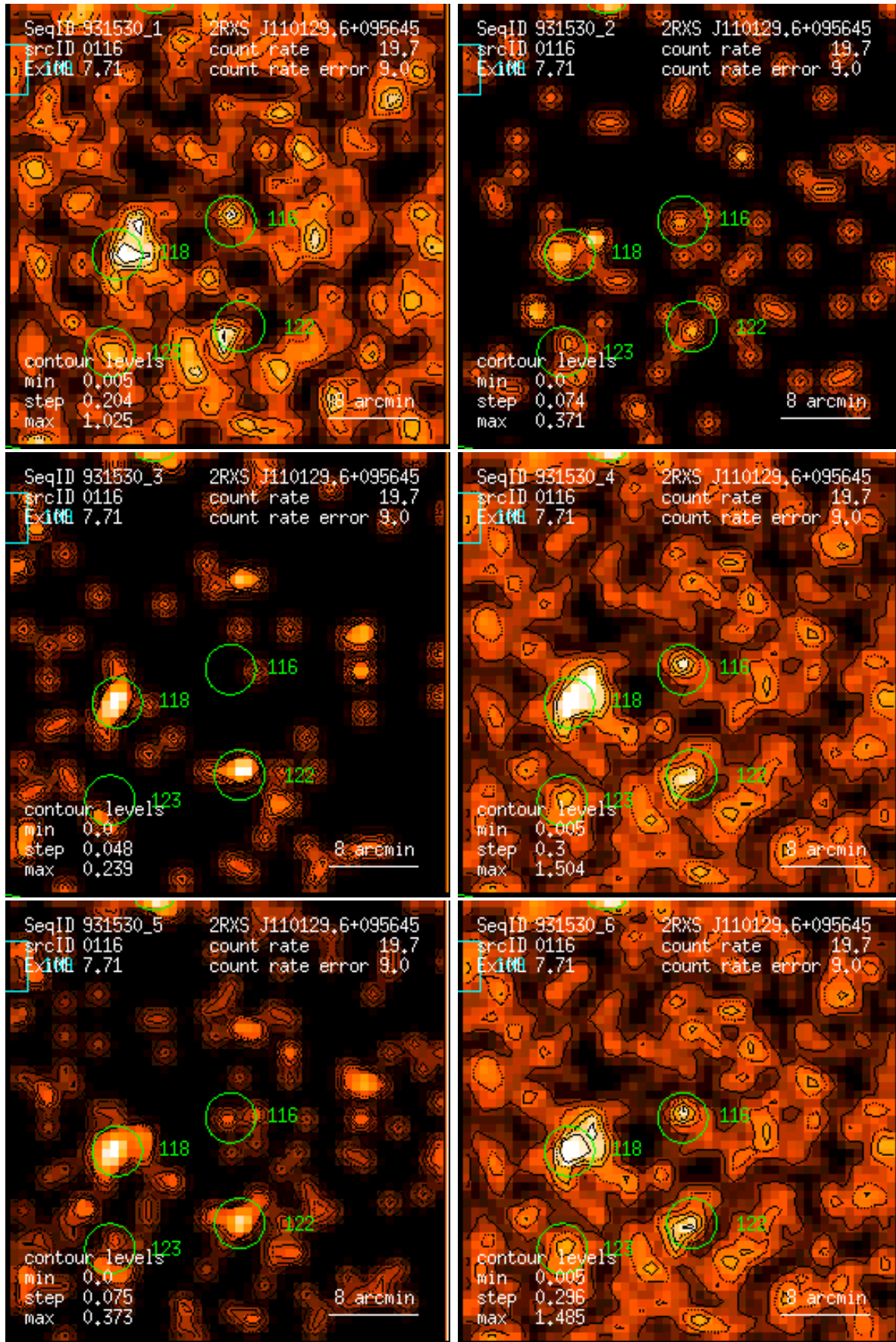
Figure 116: RASS 931530: detection 0116: band rate images, Gaussian filter: (1) PSPC channels 11 – 41, (2) 52 – 90, (3) 91 – 201, (4) 11 – 235, (5) 52 – 201, (6) 11 – 201. Broad band rates in counts/ks. Band rate contour levels in counts/ks/arcmin 2 .
