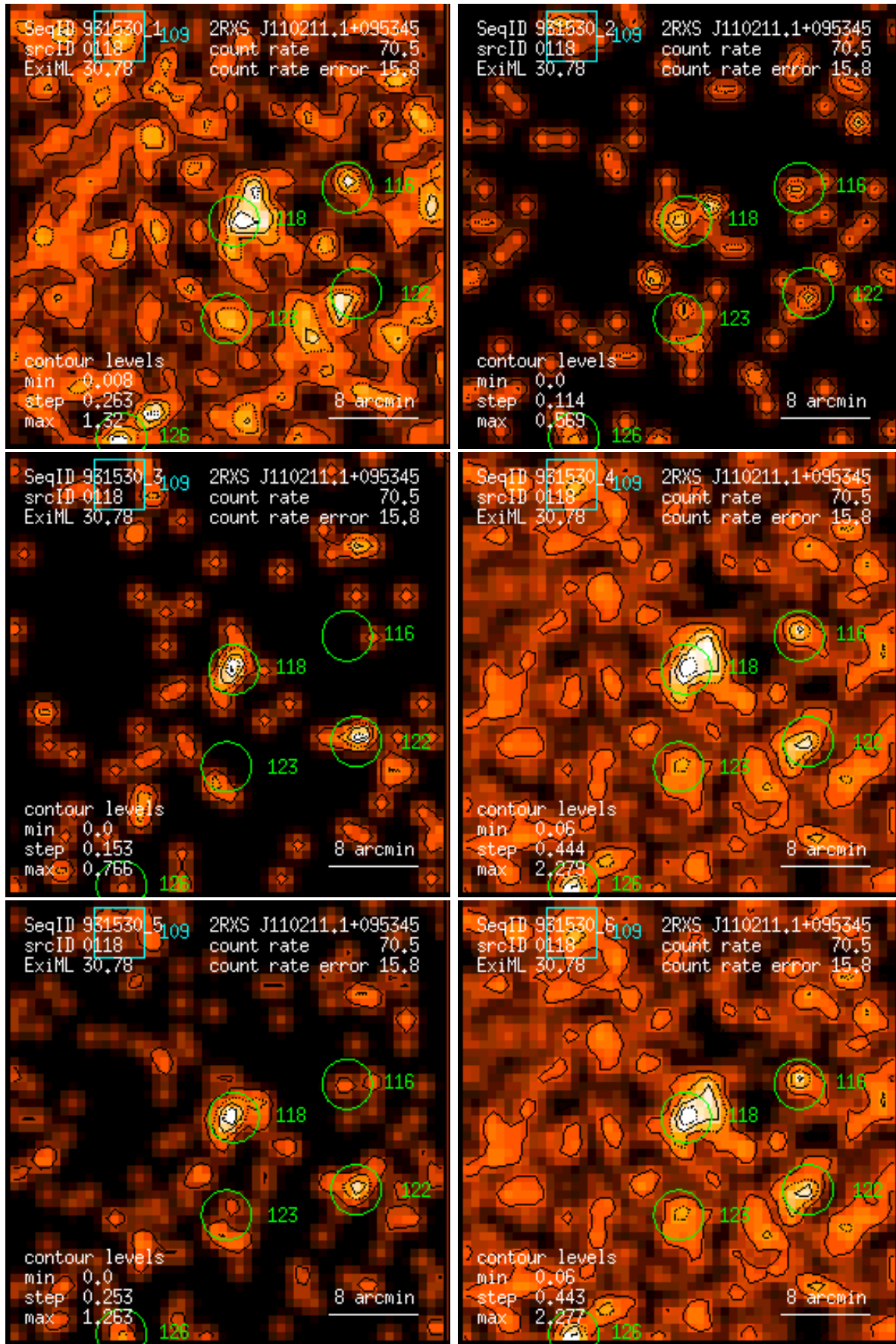
Figure 118: RASS 931530: detection 0118: band rate images, Gaussian filter: (1) PSPC channels 11 – 41, (2) 52 – 90, (3) 91 – 201, (4) 11 – 235, (5) 52 – 201, (6) 11 – 201. Broad band rates in counts/ks. Band rate contour levels in counts/ks/arcmin 2 .
