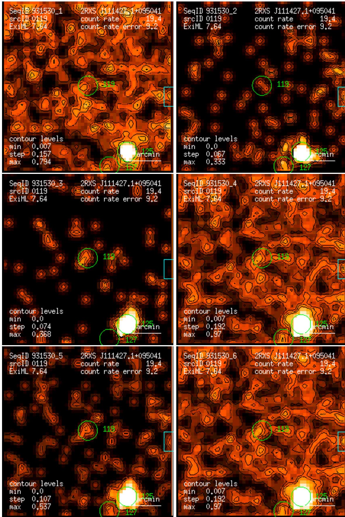
Figure 119: RASS 931530: detection 0119: band rate images, Gaussian filter: (1) PSPC channels 11 – 41, (2) 52 – 90, (3) 91 – 201, (4) 11 – 235, (5) 52 – 201, (6) 11 – 201. Broad band rates in counts/ks. Band rate contour levels in counts/ks/arcmin 2 .
