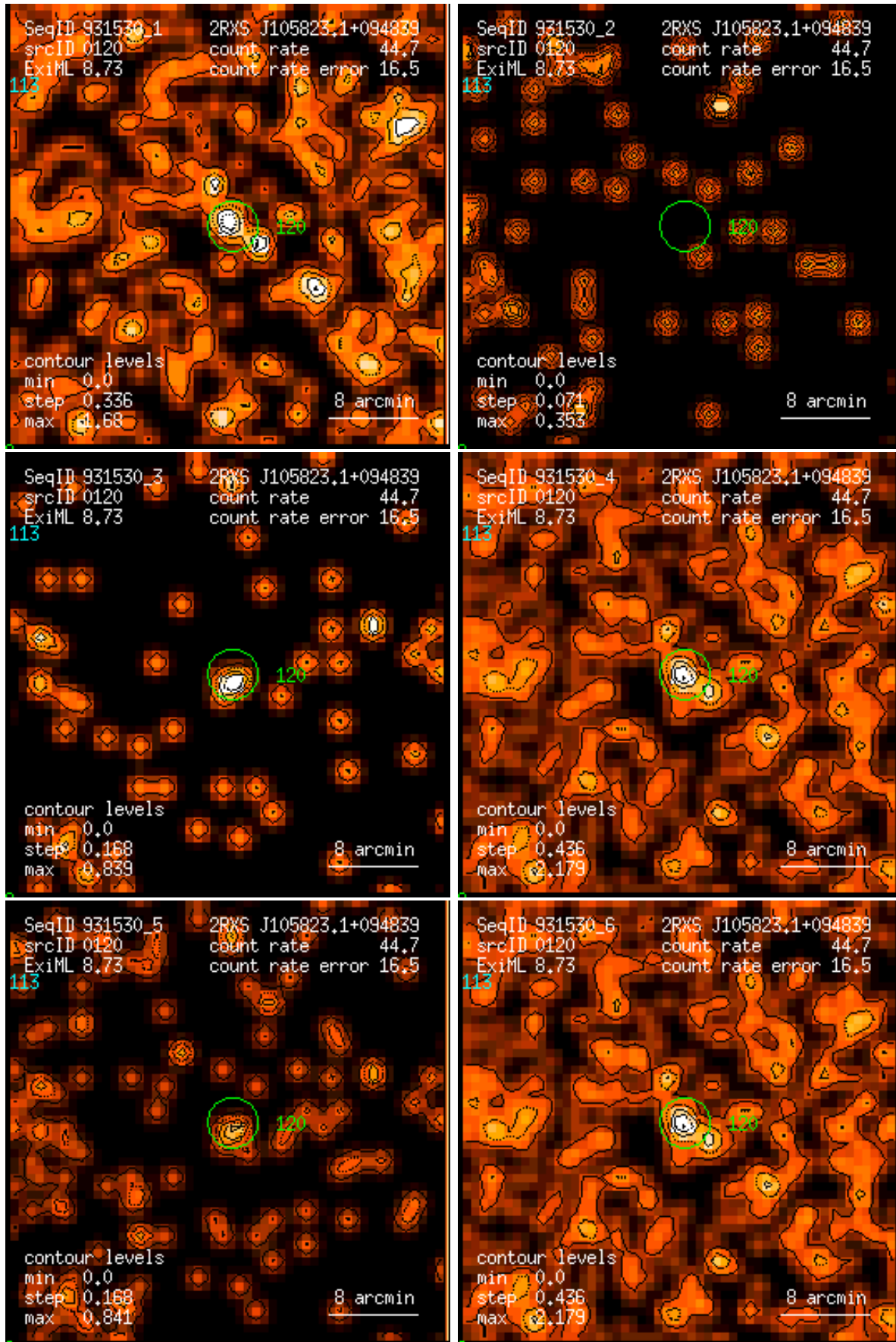
Figure 120: RASS 931530: detection 0120: band rate images, Gaussian filter: (1) PSPC channels 11 – 41, (2) 52 – 90, (3) 91 – 201, (4) 11 – 235, (5) 52 – 201, (6) 11 – 201. Broad band rates in counts/ks. Band rate contour levels in counts/ks/arcmin 2 .
