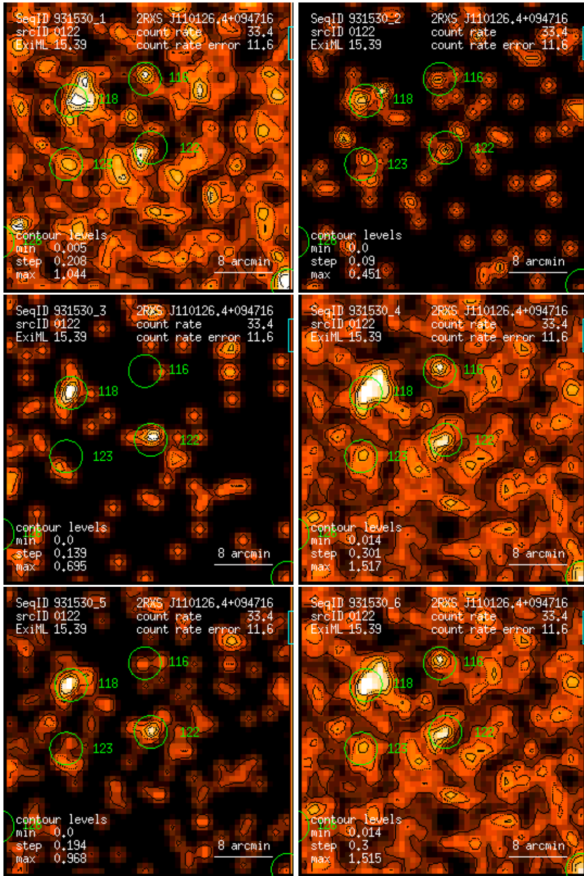
Figure 122: RASS 931530: detection 0122: band rate images, Gaussian filter: (1) PSPC channels 11 – 41, (2) 52 – 90, (3) 91 – 201, (4) 11 – 235, (5) 52 – 201, (6) 11 – 201. Broad band rates in counts/ks. Band rate contour levels in counts/ks/arcmin 2 .
