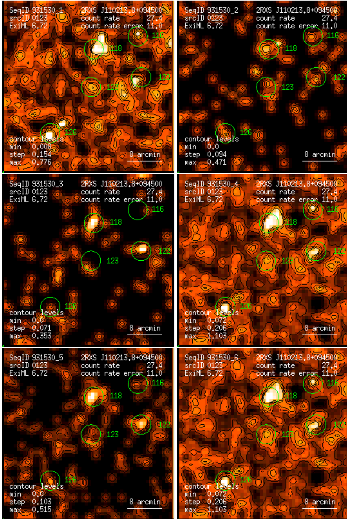
Figure 123: RASS 931530: detection 0123: band rate images, Gaussian filter: (1) PSPC channels 11 – 41, (2) 52 – 90, (3) 91 – 201, (4) 11 – 235, (5) 52 – 201, (6) 11 – 201. Broad band rates in counts/ks. Band rate contour levels in counts/ks/arcmin 2 .
