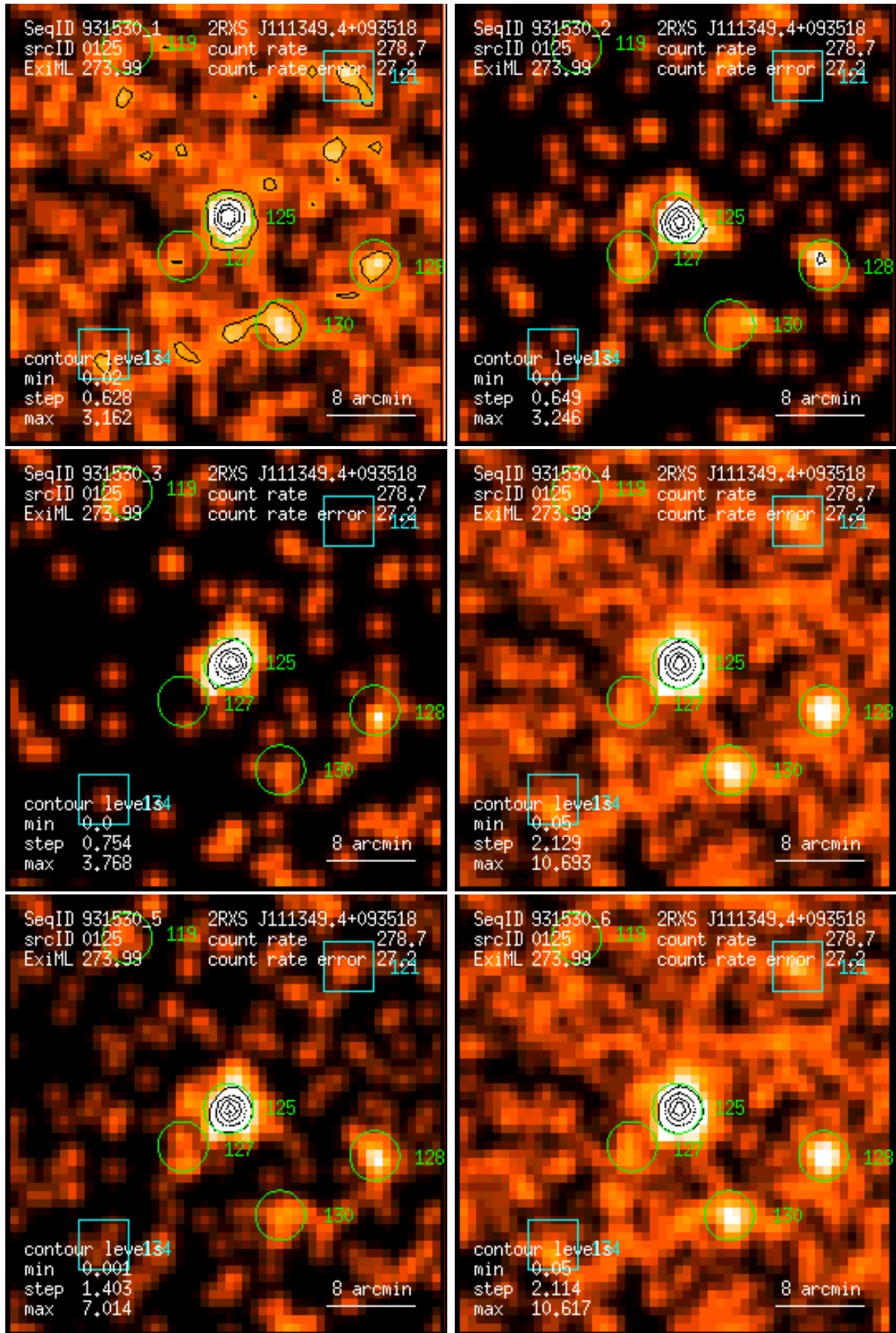
Figure 125: RASS 931530: detection 0125: band rate images, Gaussian filter: (1) PSPC channels 11 – 41, (2) 52 – 90, (3) 91 – 201, (4) 11 – 235, (5) 52 – 201, (6) 11 – 201. Broad band rates in counts/ks. Band rate contour levels in counts/ks/arcmin 2 .
