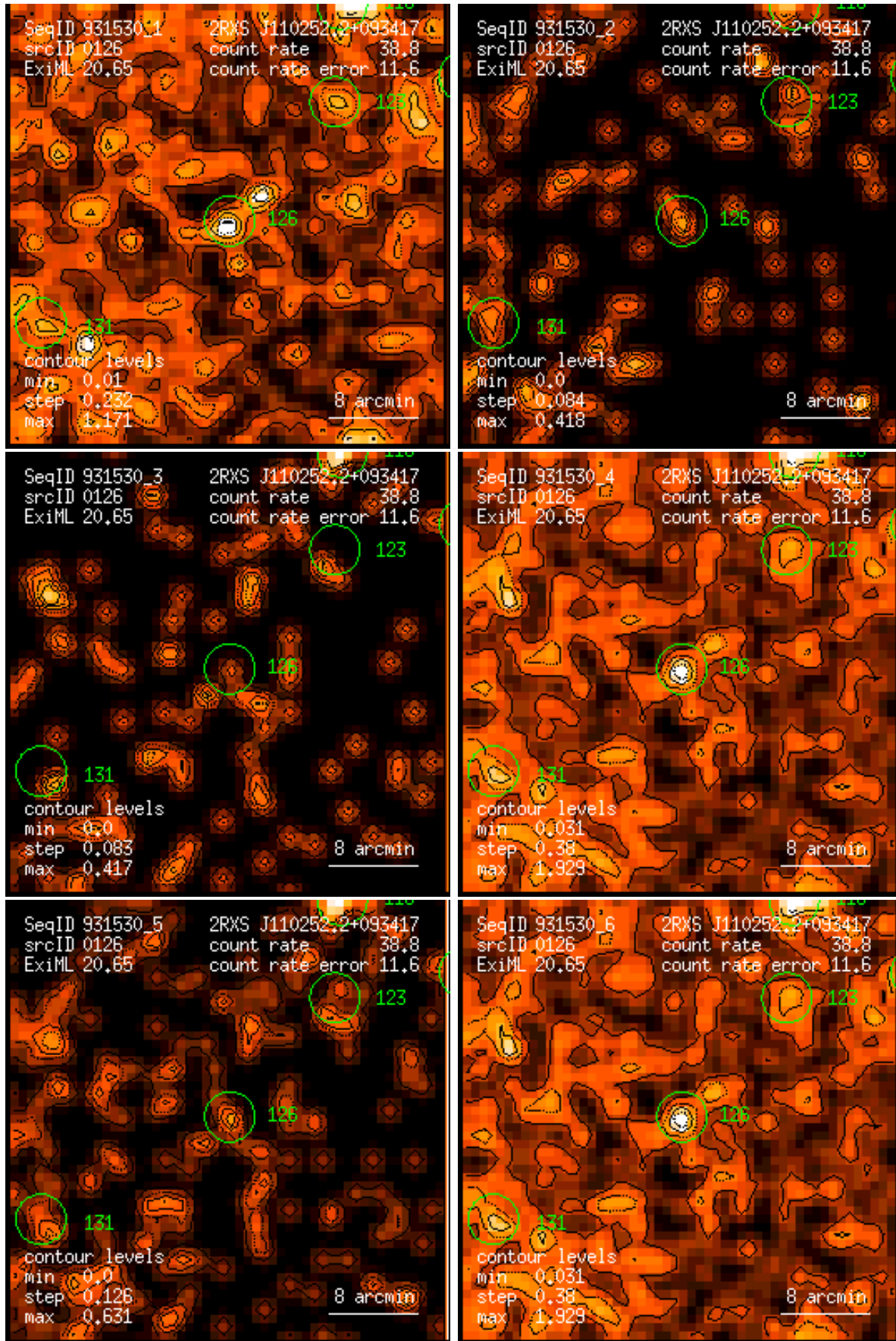
Figure 126: RASS 931530: detection 0126: band rate images, Gaussian filter: (1) PSPC channels 11 – 41, (2) 52 – 90, (3) 91 – 201, (4) 11 – 235, (5) 52 – 201, (6) 11 – 201. Broad band rates in counts/ks. Band rate contour levels in counts/ks/arcmin 2 .
