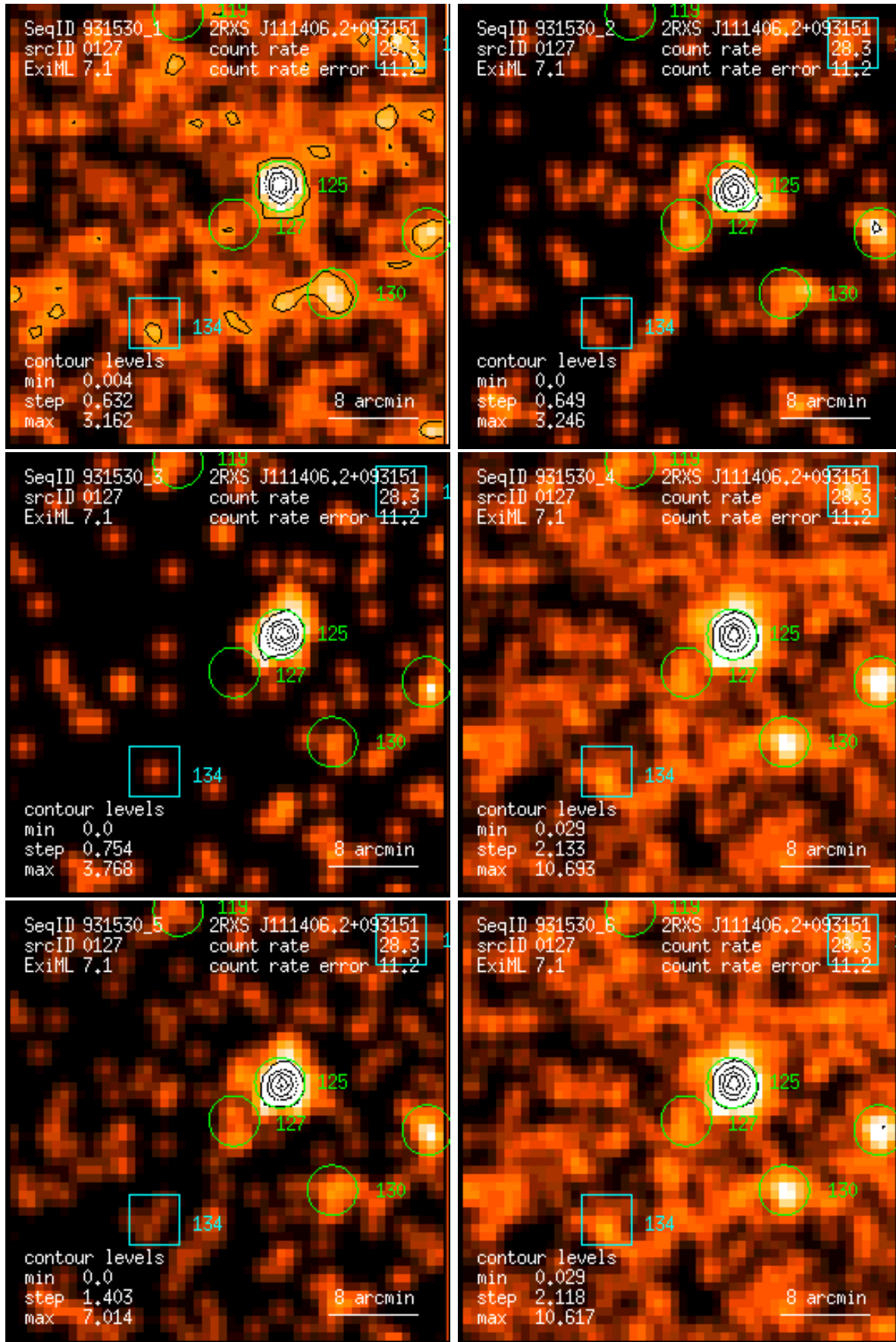
Figure 127: RASS 931530: detection 0127: band rate images, Gaussian filter: (1) PSPC channels 11 – 41, (2) 52 – 90, (3) 91 – 201, (4) 11 – 235, (5) 52 – 201, (6) 11 – 201. Broad band rates in counts/ks. Band rate contour levels in counts/ks/arcmin 2 .
