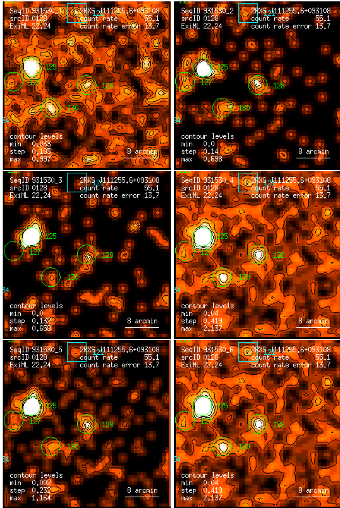
Figure 128: RASS 931530: detection 0128: band rate images, Gaussian filter: (1) PSPC channels 11 – 41, (2) 52 – 90, (3) 91 – 201, (4) 11 – 235, (5) 52 – 201, (6) 11 – 201. Broad band rates in counts/ks. Band rate contour levels in counts/ks/arcmin 2 .
