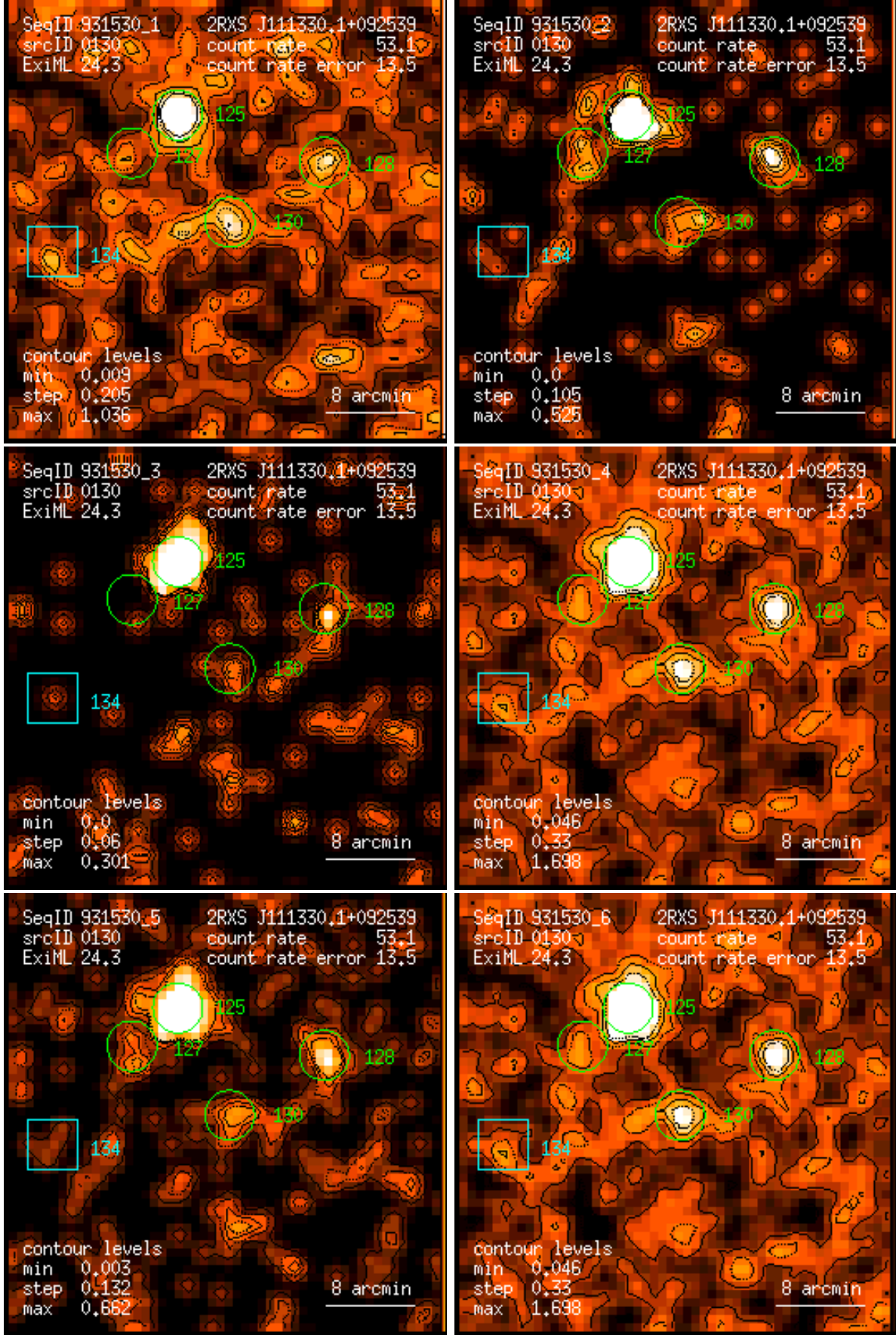
Figure 130: RASS 931530: detection 0130: band rate images, Gaussian filter: (1) PSPC channels 11 – 41, (2) 52 – 90, (3) 91 – 201, (4) 11 – 235, (5) 52 – 201, (6) 11 – 201. Broad band rates in counts/ks. Band rate contour levels in counts/ks/arcmin 2 .
