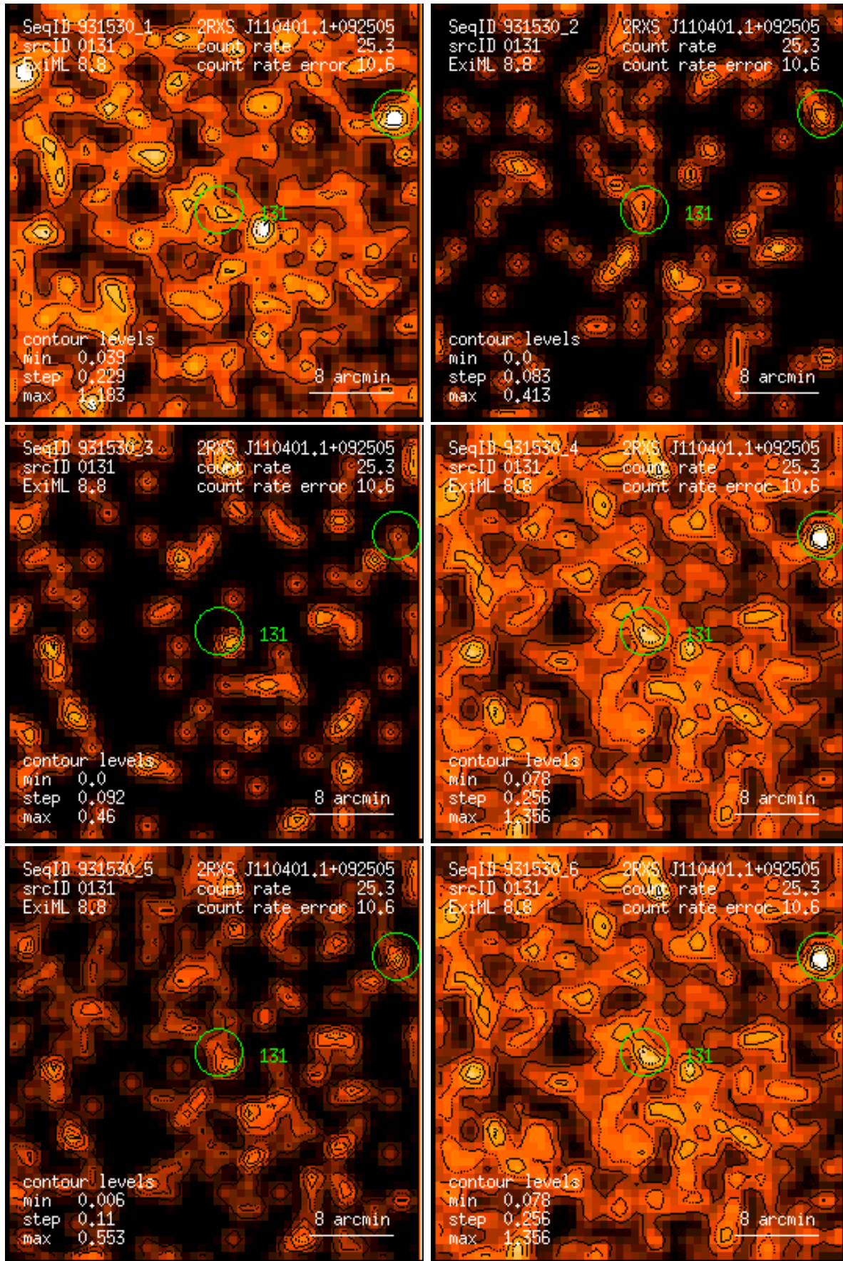
Figure 131: RASS 931530: detection 0131: band rate images, Gaussian filter: (1) PSPC channels 11 – 41, (2) 52 – 90, (3) 91 – 201, (4) 11 – 235, (5) 52 – 201, (6) 11 – 201. Broad band rates in counts/ks. Band rate contour levels in counts/ks/arcmin 2 .
